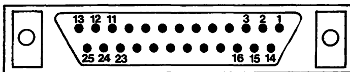
Figure F-1. RS232C Connector Pin Assignment
