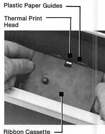
Figure 2-2. Lining Up the Ribbon Cassette
