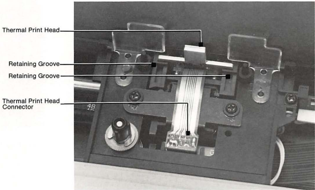
Figure 5-1. Thermal Print Head Removal
