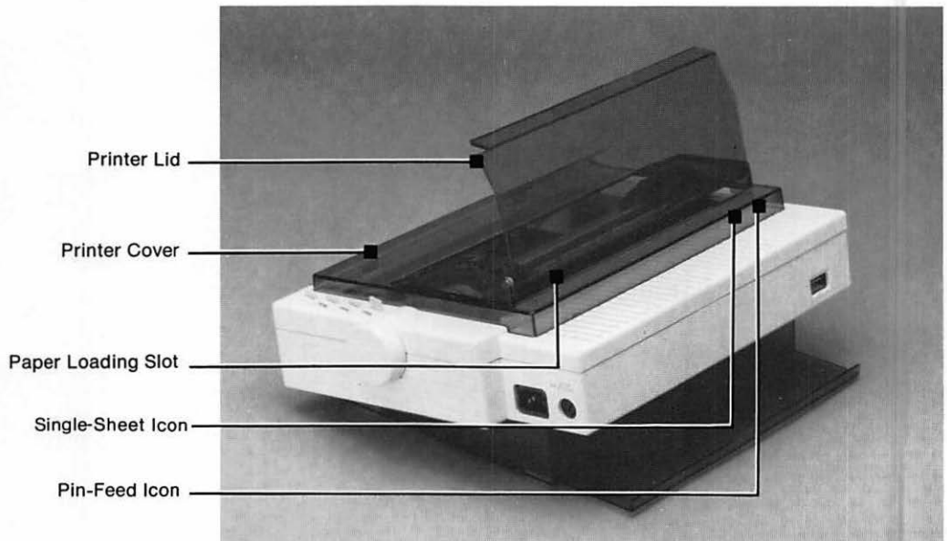
Figure 1-2. Printer Cover
