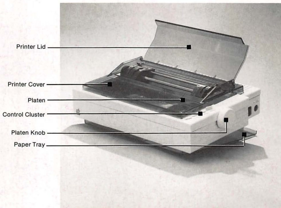
Figure 1-1. Front View
