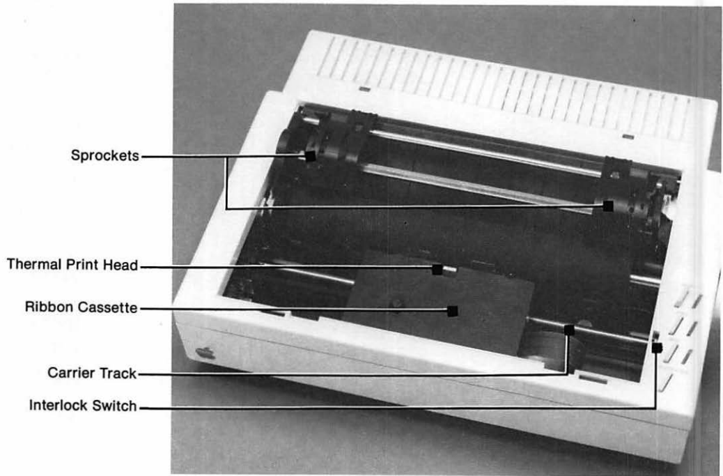
Figure 1-9. Scribe Interior
