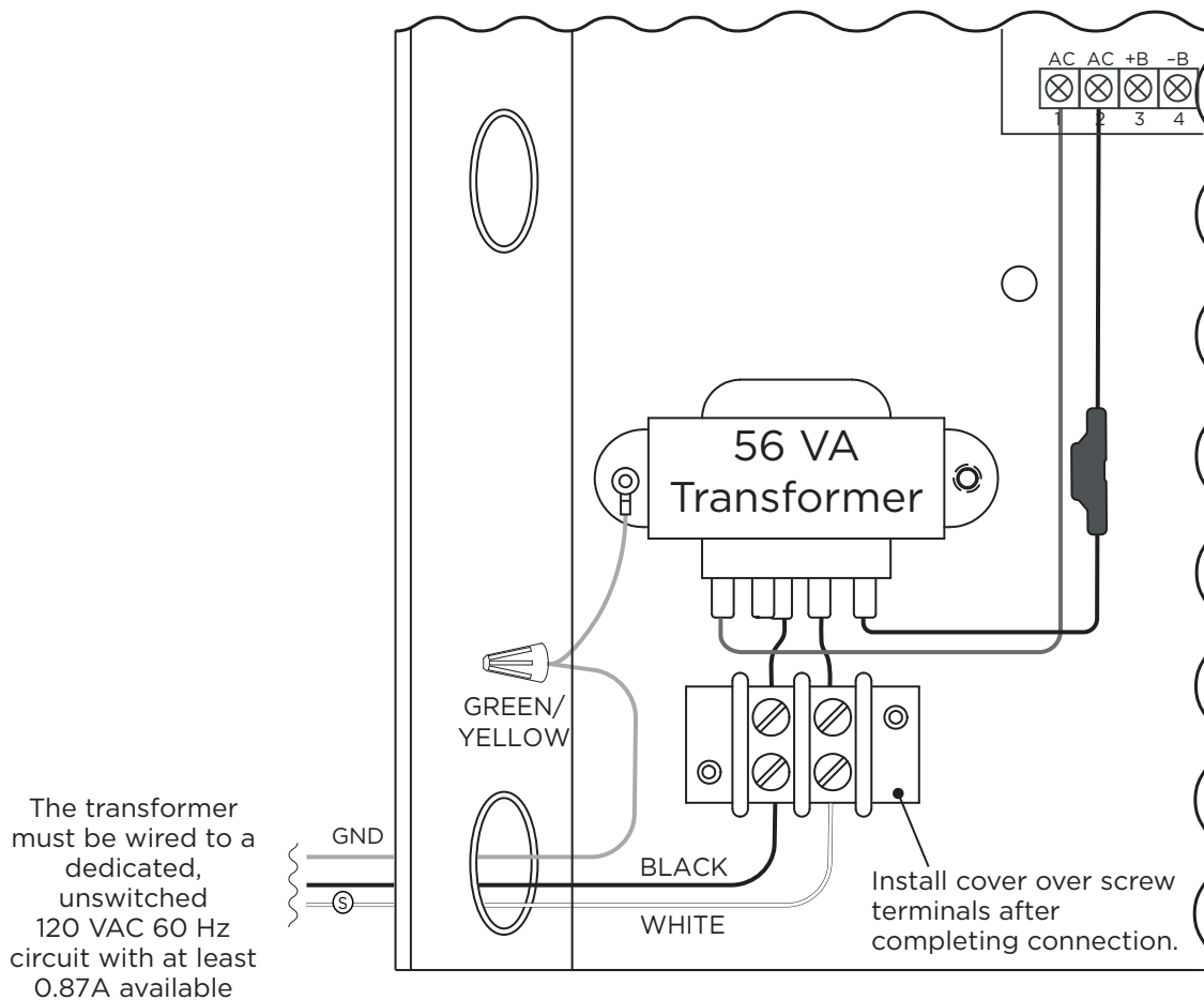
Figure 4: Transformer Wiring
