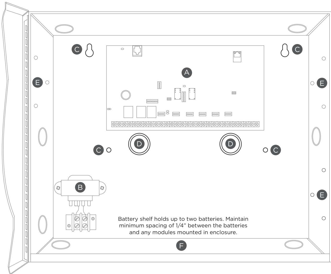
Figure 2: XR150FC/XR550FC Enclosure
