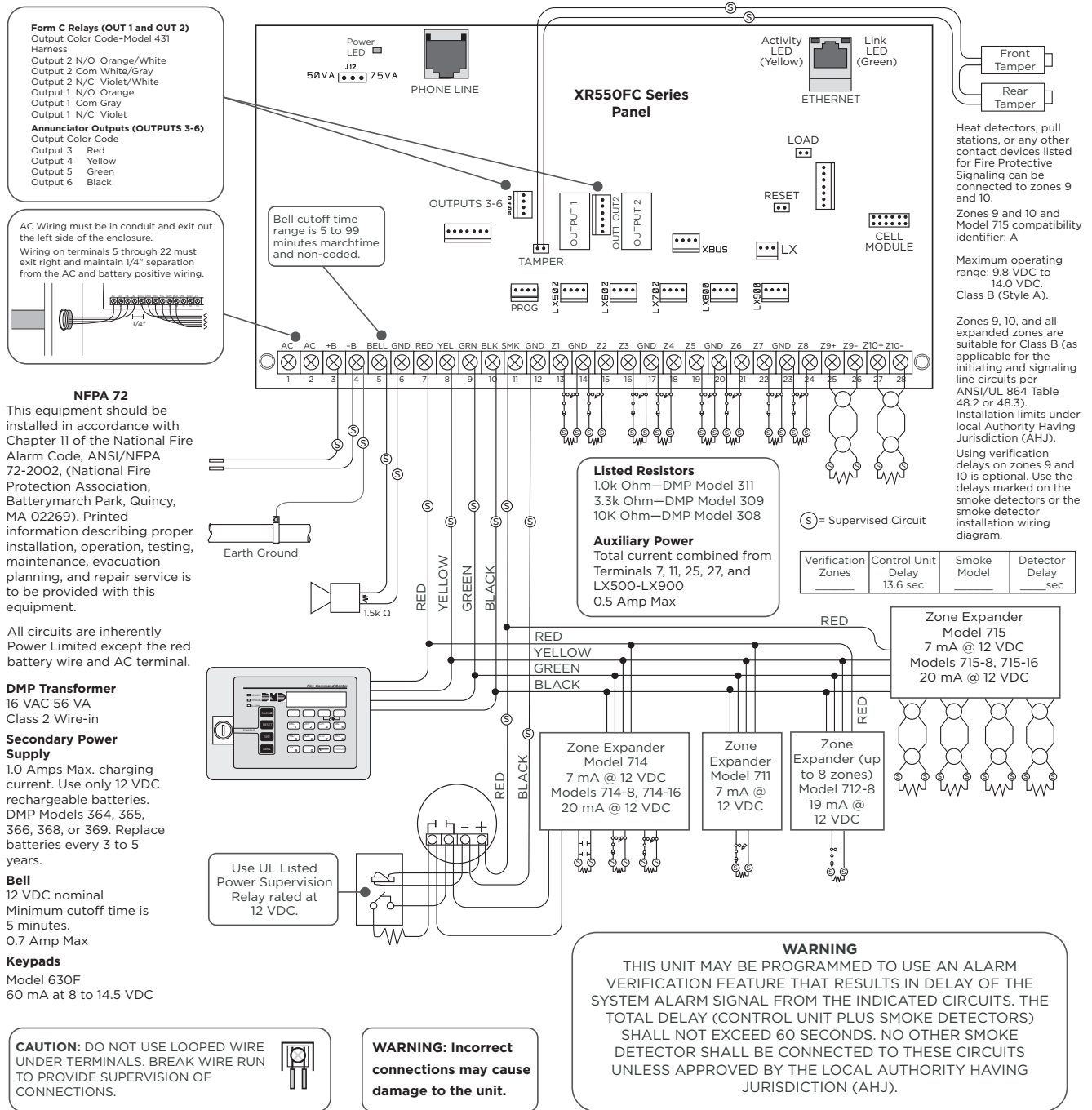
Figure 1: XR150FC/XR550FC Series Wiring Diagram
