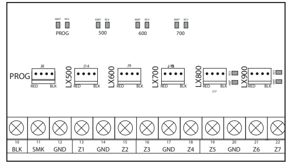
Figure 6: LX-Bus Headers and LEDs
