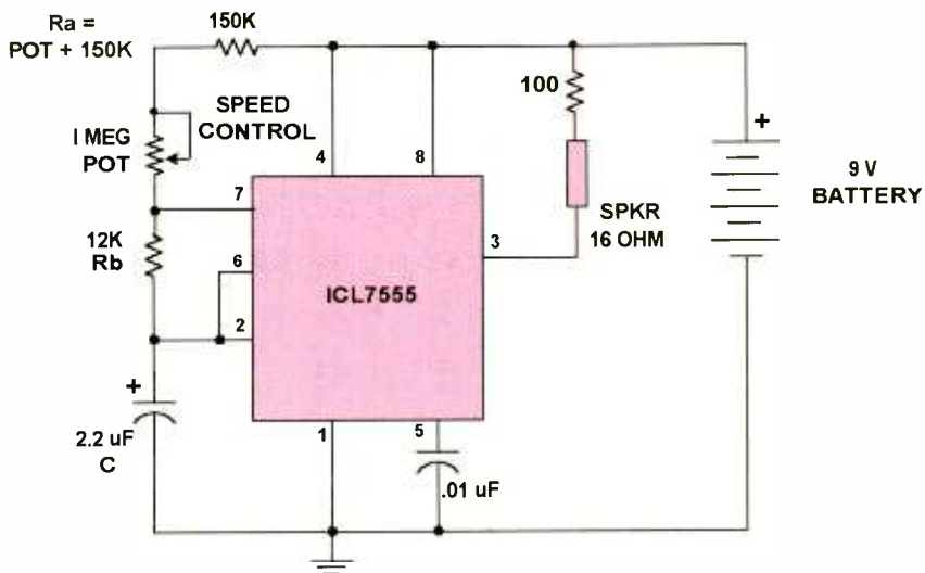
FIG 2 METRONOME CIRCUIT
