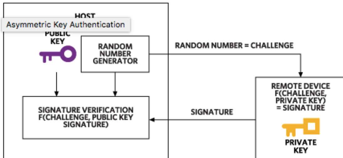
Figure 2: Asymmetric key authentication relies on public and private keys.
