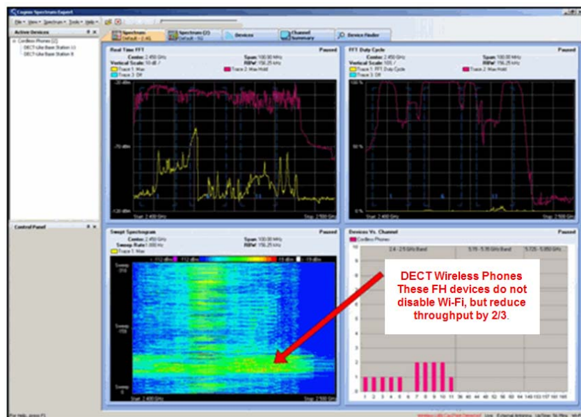
Figure 37 Display that shows 2.4 GHz interference from DECT phones
