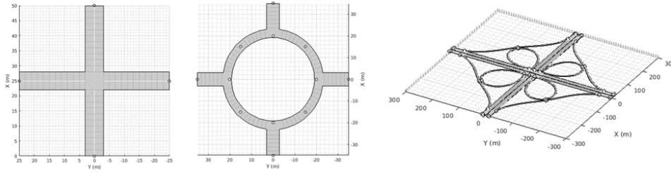
Figure 10:- Examples of ADAS generated roadways 2
