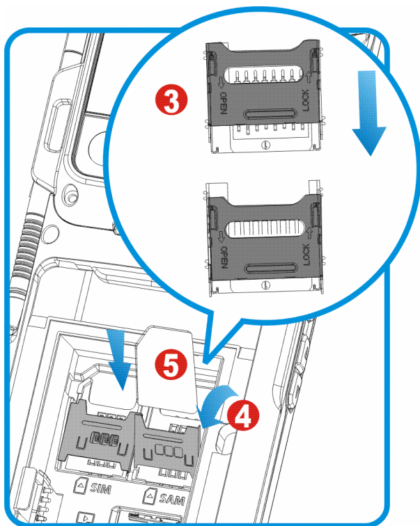
Figure 19: Inserting SAM Card
