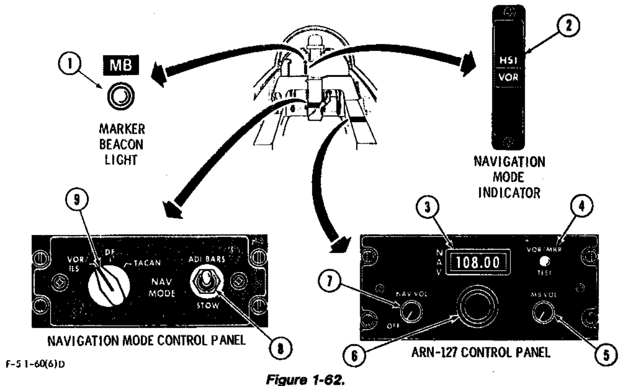
NAVIGATION CONTROLS/INDICATORS (Figure 1-62)
