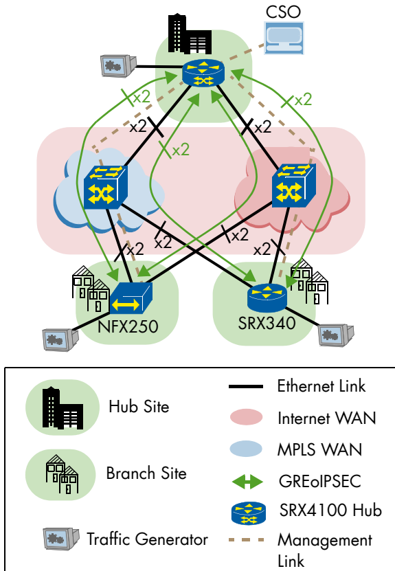
Figure 8: Logical Topology Used for Application-based Traffic Steering Scenarios
