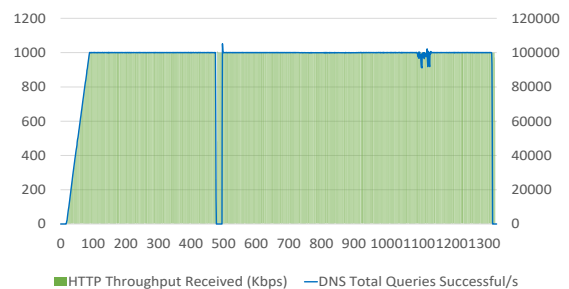
Figure 10: Primary Hub Failure HTTP Throughput and DNS Total Successful Queries
