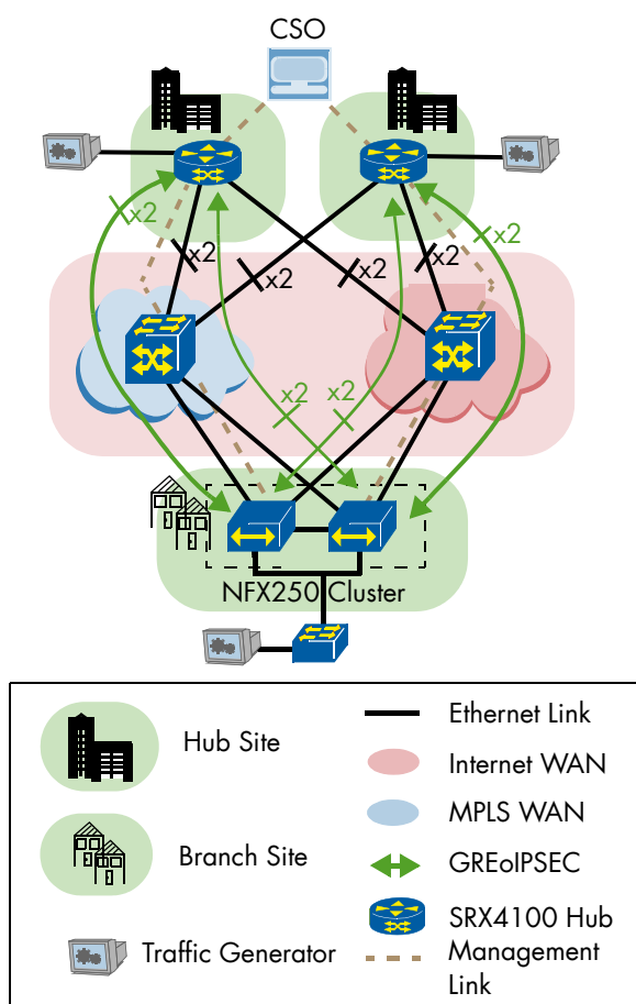
Figure 5: Dual-CPE Multi-Homing Topology
