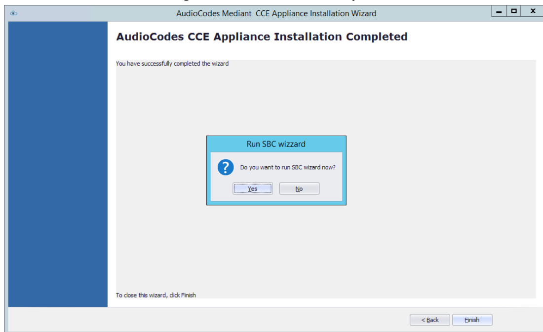
Figure 4-36: Installation Complete
