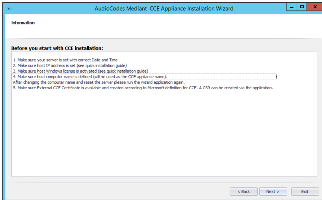
Figure 4-16: Prerequisites
