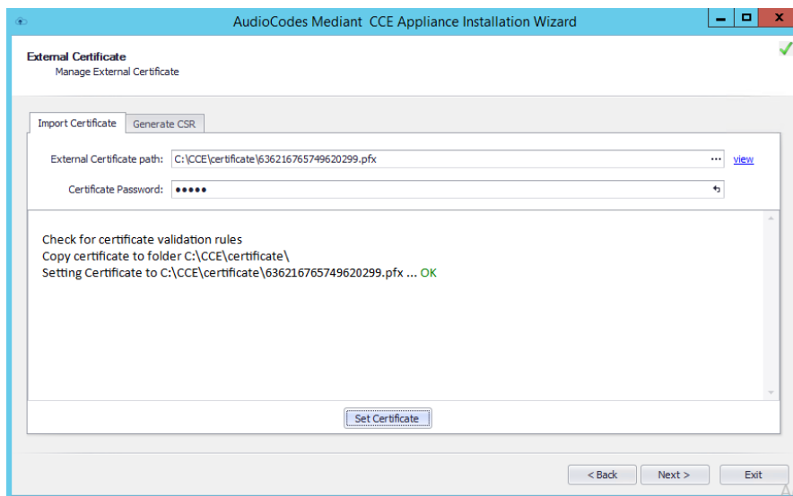
Figure 4-23: Import Certificate
