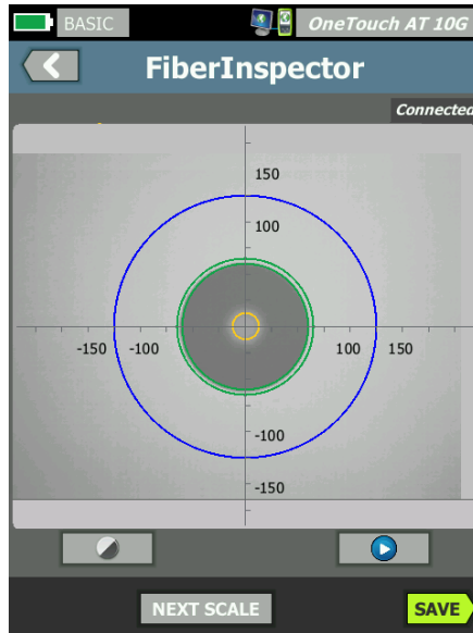
Figure 73. FiberInspector Image with Measurement Scales (fiber with 50 \mu\text{m} core shown)
