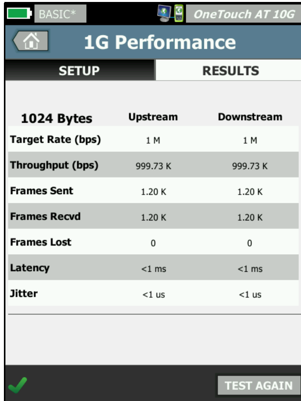
Figure 41. 1G Wired Performance Test (RFC 2544) Results Using a Single Frame Size
