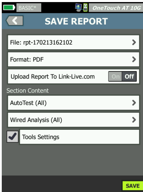
Figure 76. Save Report Screen—Possible Report Options
