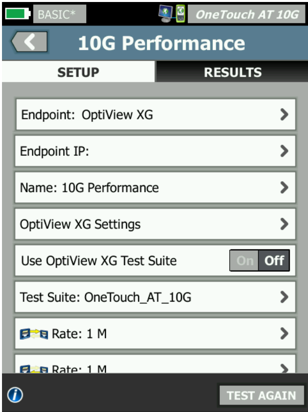
Figure 44. 10G Wired Performance Test Setup Tab Using OptiView XG
