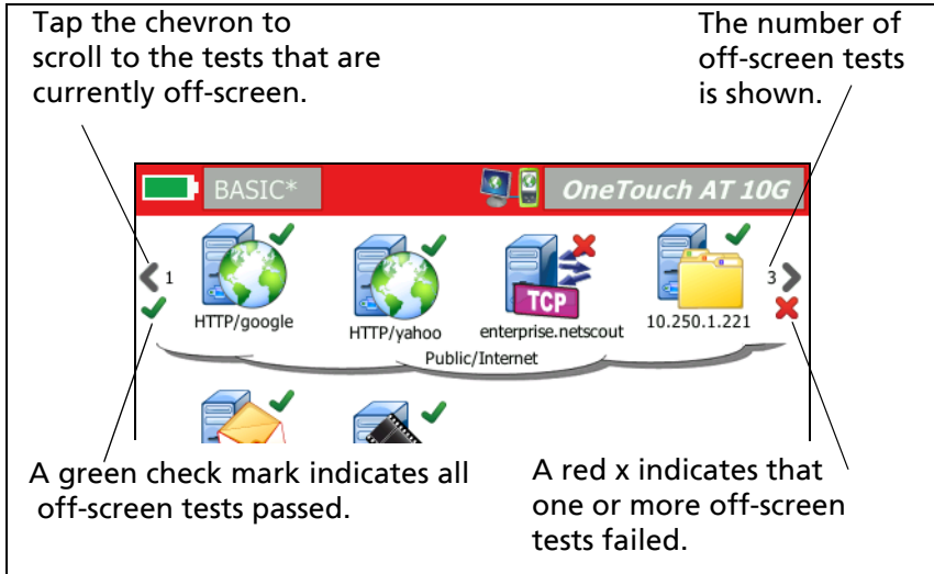
Figure 24. Seeing Off-Screen Tests
