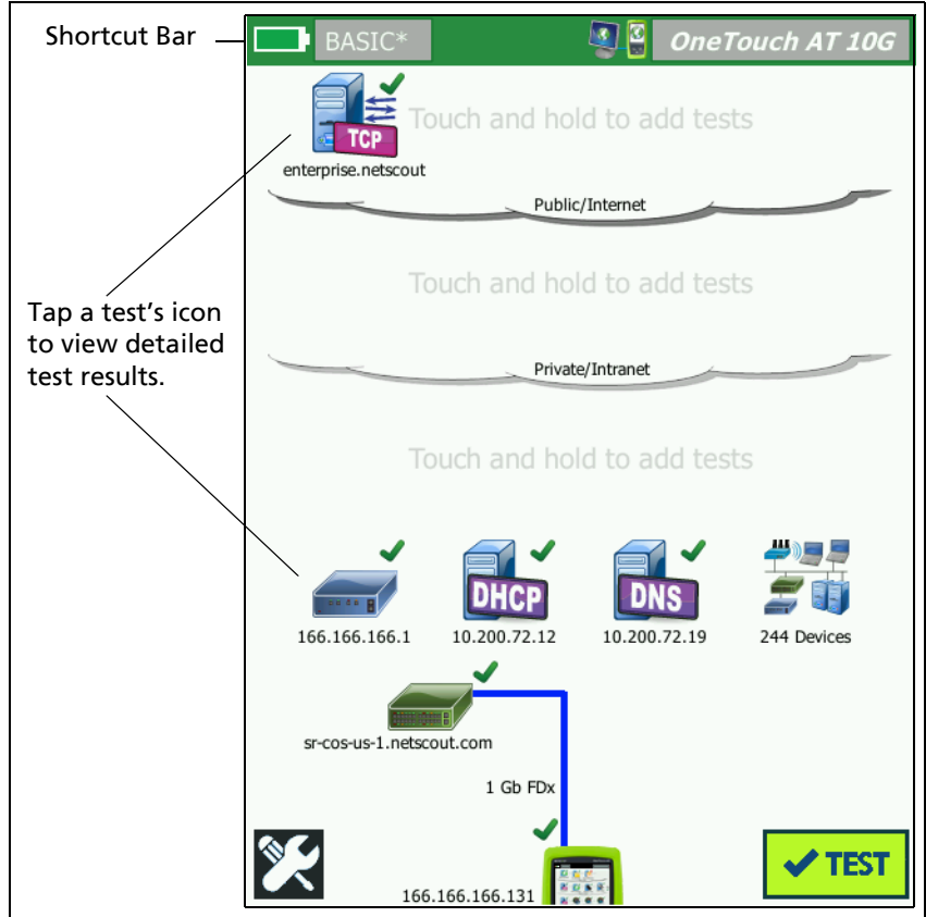
Figure 22. HOME Screen After Running AutoTest
