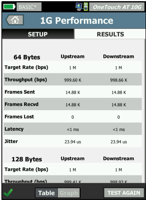
Figure 42. 1G Wired Performance Test (RFC 2544) Results RFC 2544 Sweep, Tabular View
