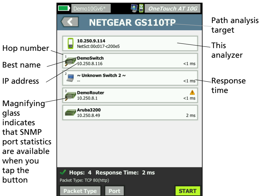
Figure 59. Path Analysis Results
