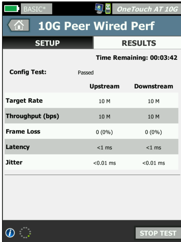
Figure 48. 10G Performance (Y.1564) test - full performance test phase
