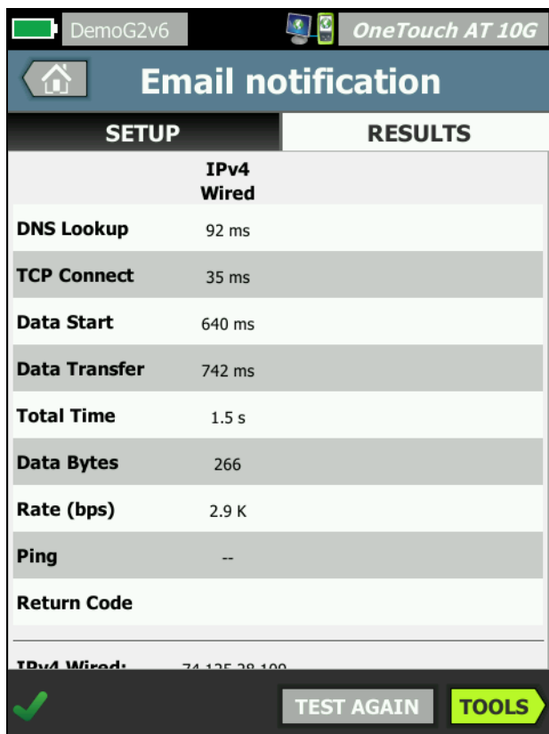
Figure 51. Email (SMTP) Test Results
