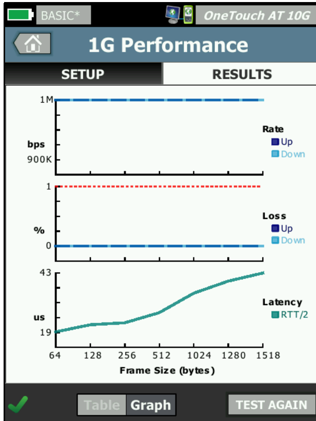
Figure 43. Wired Performance Test Results RFC 2544 sweep, Graphical View
