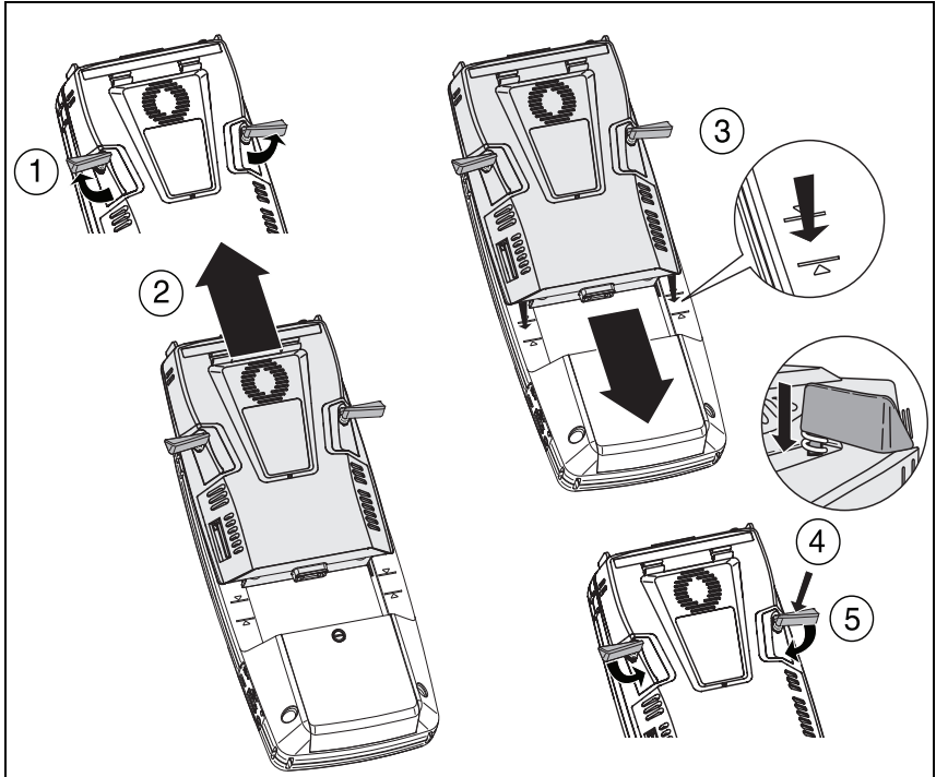
Figure 2. Remove and Install a Module
