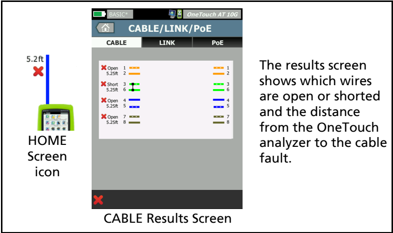
Figure 27. Underterminated Cable with Shorts and Opens
