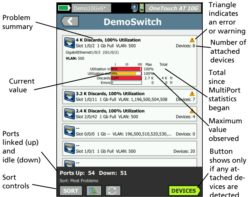
Figure 64. MultiPort Statistics Details Screen
