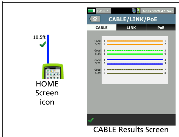
Figure 26. Untermated Cable
