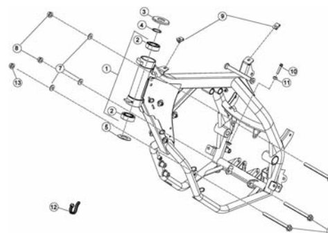
TAV.31 Telaio - Frame - Chassis - Rahmen - Chasis
