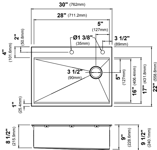
Model #: KWT310-30 Sink Dimensions: 30" x 22" x 9" Min Cabinet Size: 33"
