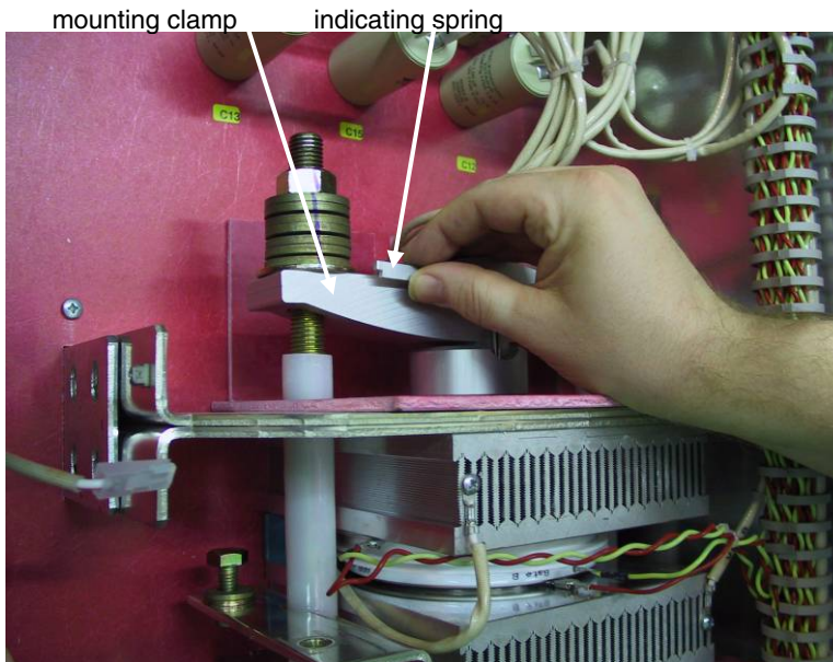
Handling of indicating spring and mounting clamp
