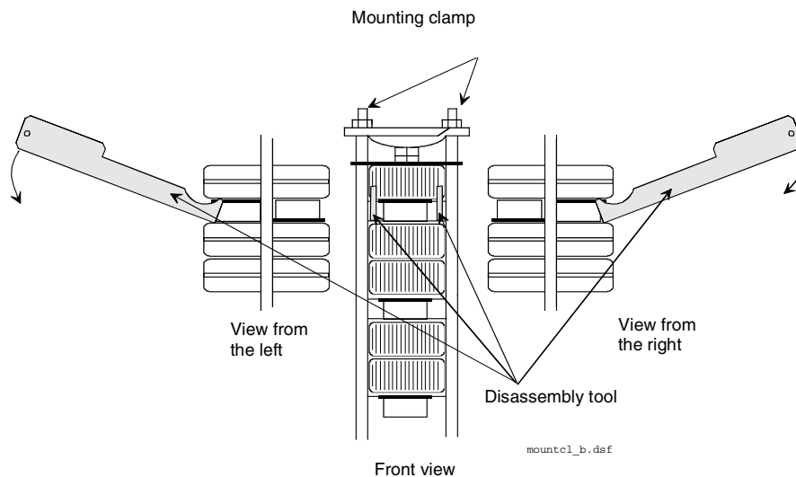
How to use the disassembly tool
