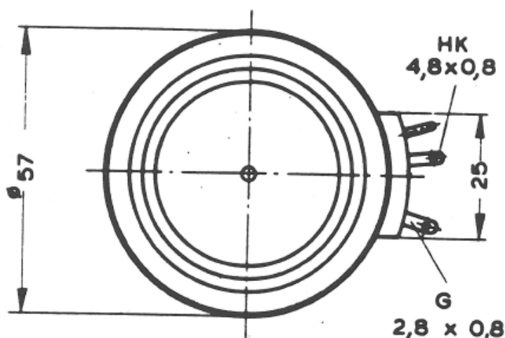
Original thyristor type
