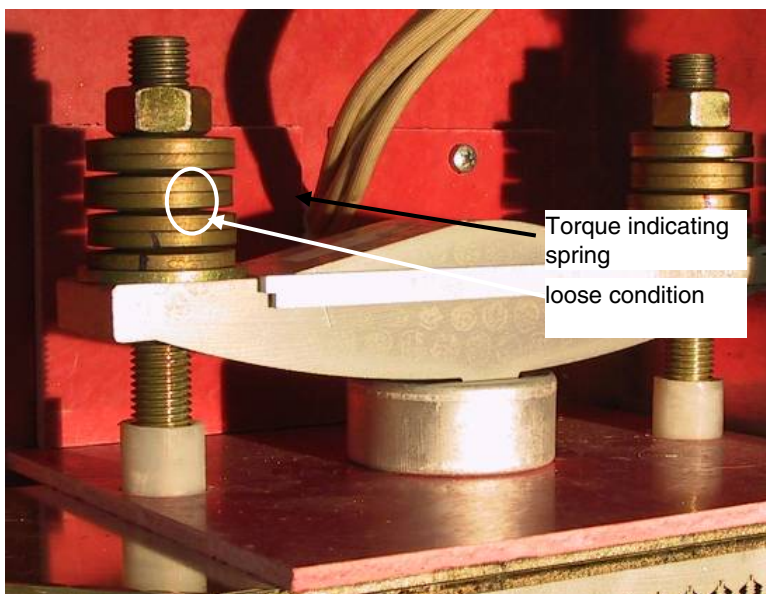
Mounting clamp; loose condition
