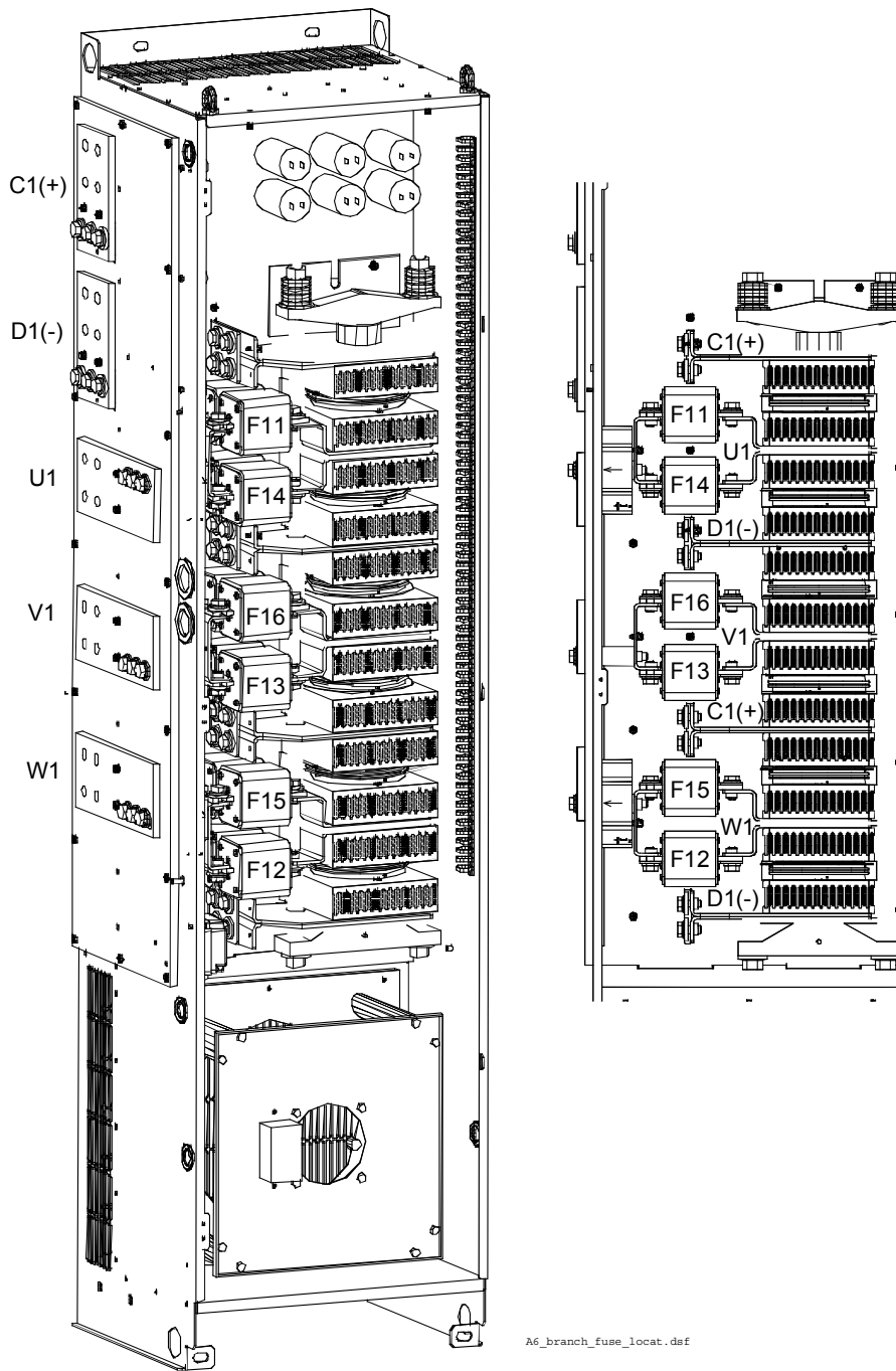
Location of parallel branch fuses frame D6
