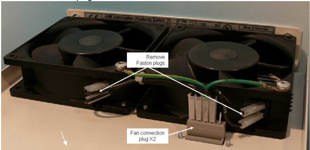
Faston plugs
