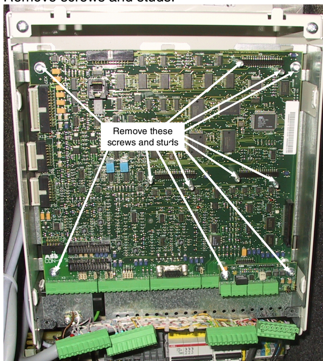
Remove screws and studs
