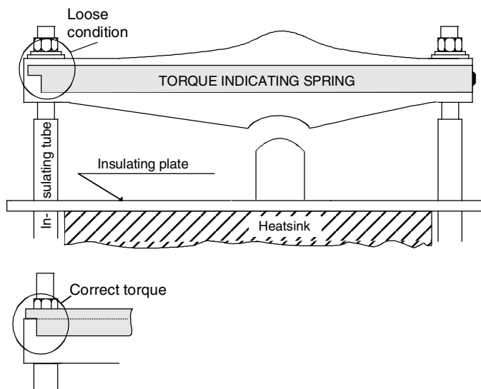
Aluminum spring with welded indicating spring
