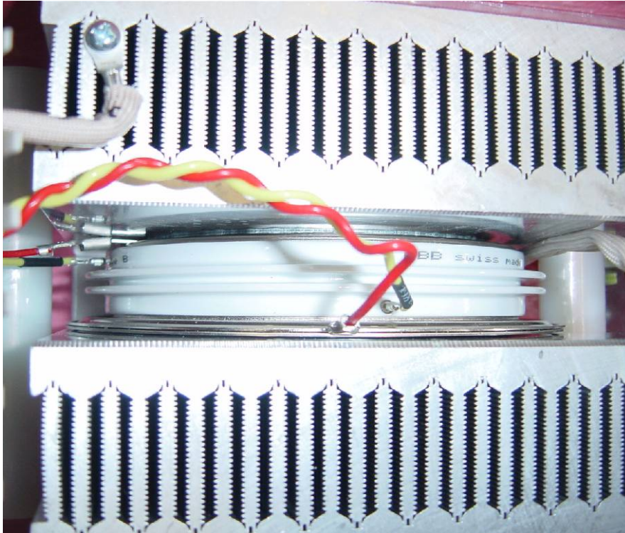
Location of BCT's gate A when built in
