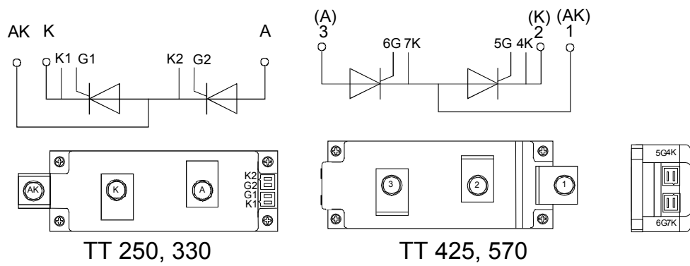
Terminals of the OnBoard bridge and all thyristor modules
