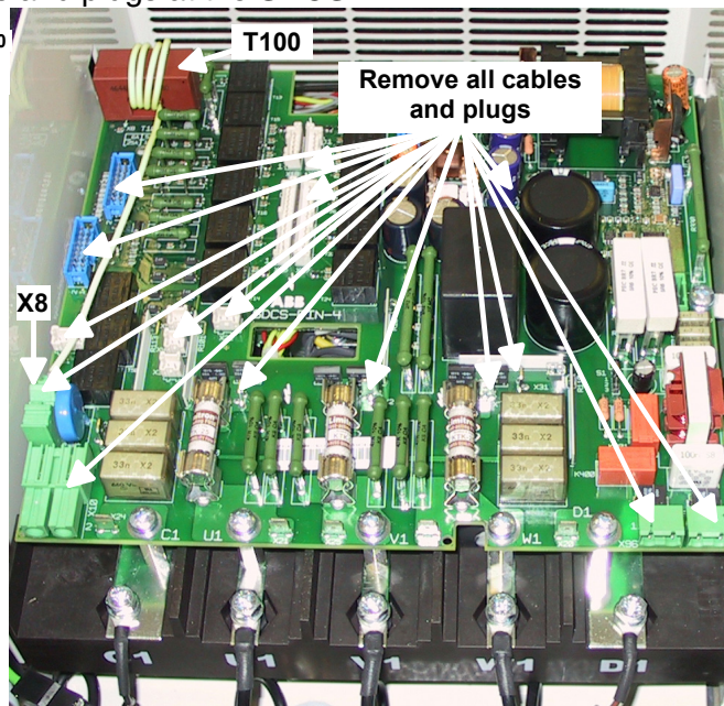
Remove cables at the SDCS-PIN-4
