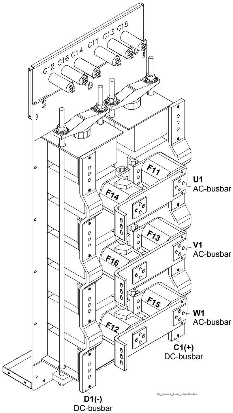
Location of branch fuses frame D7 (busbars on the left)
