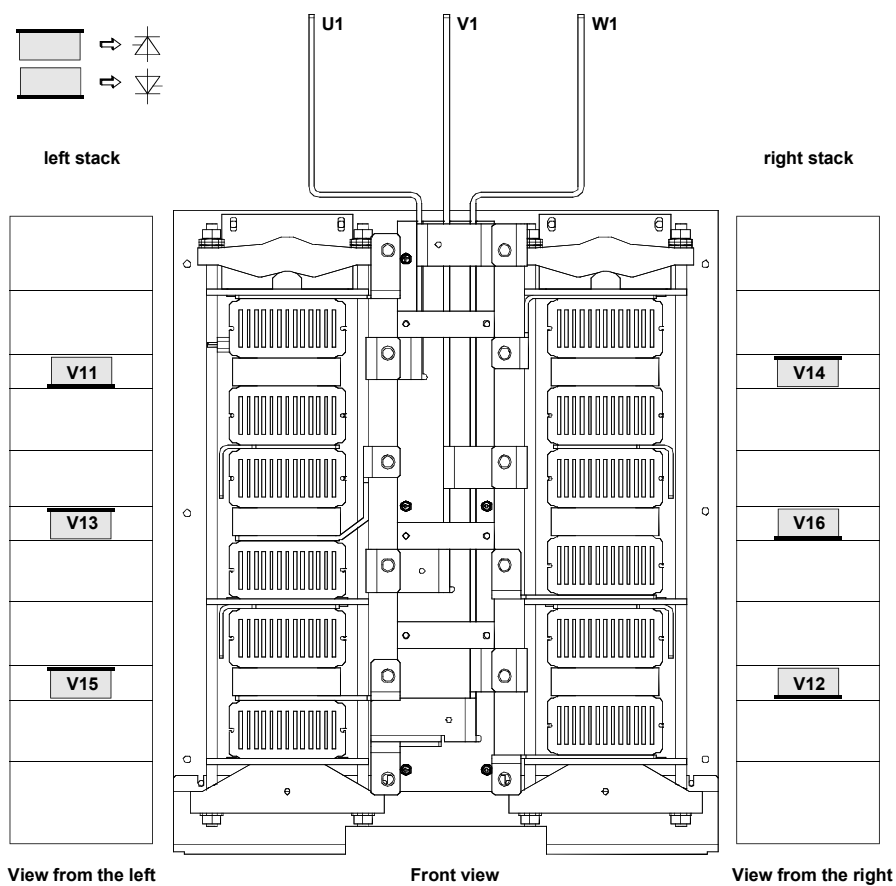
Location of thyristors in frame D5 (2-Q bridge)
