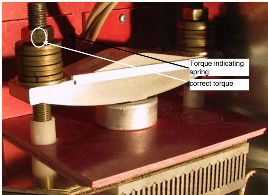
Mounting clamp, correct torque
