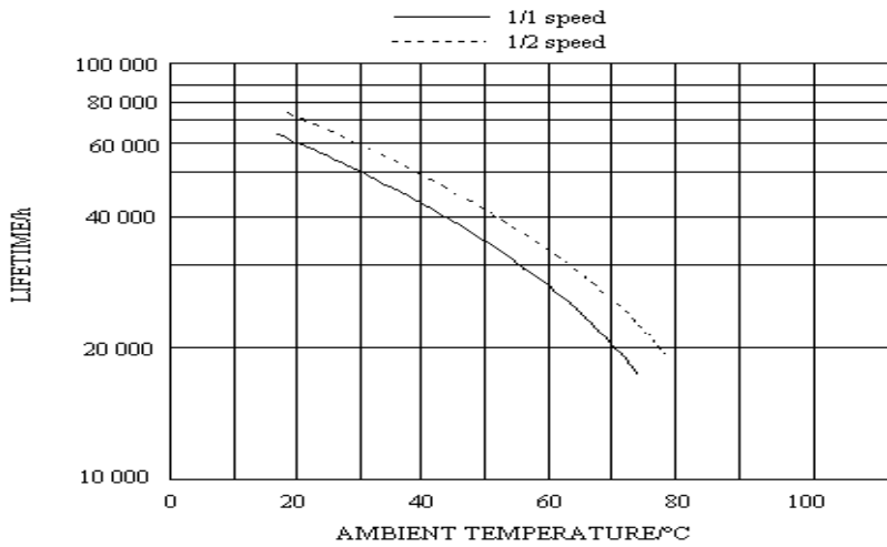
Typical lifetime of the cooling fan versus ambient temperature
