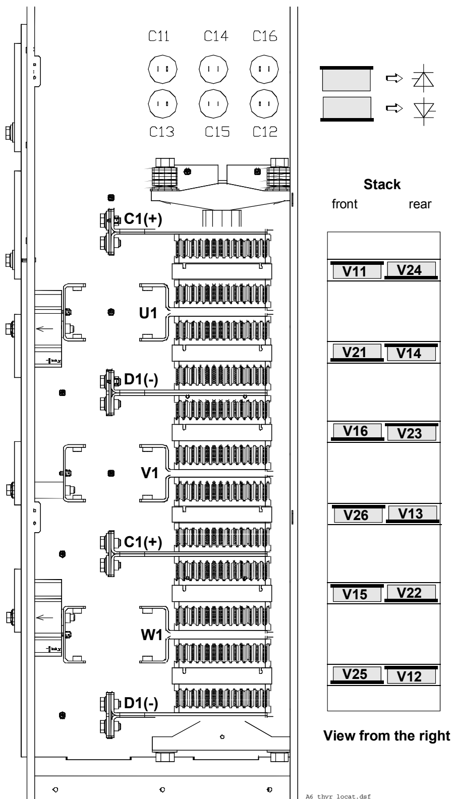
Location of thyristors in frame D6 (4-Q bridge with single thyristors)
