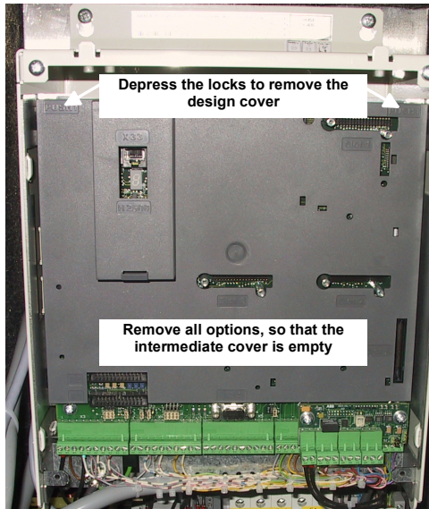
Remove plug in options
