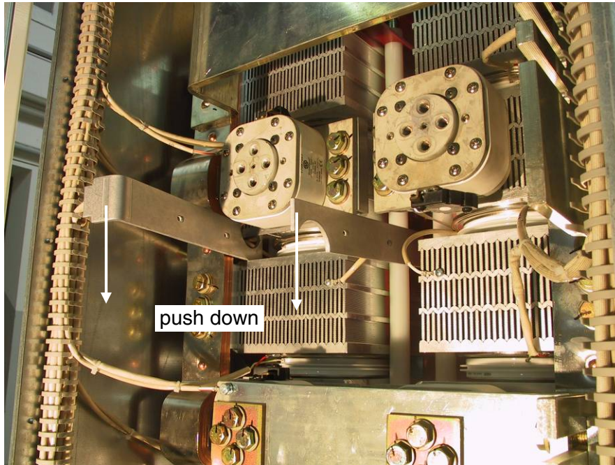
Use of disassembly tool
