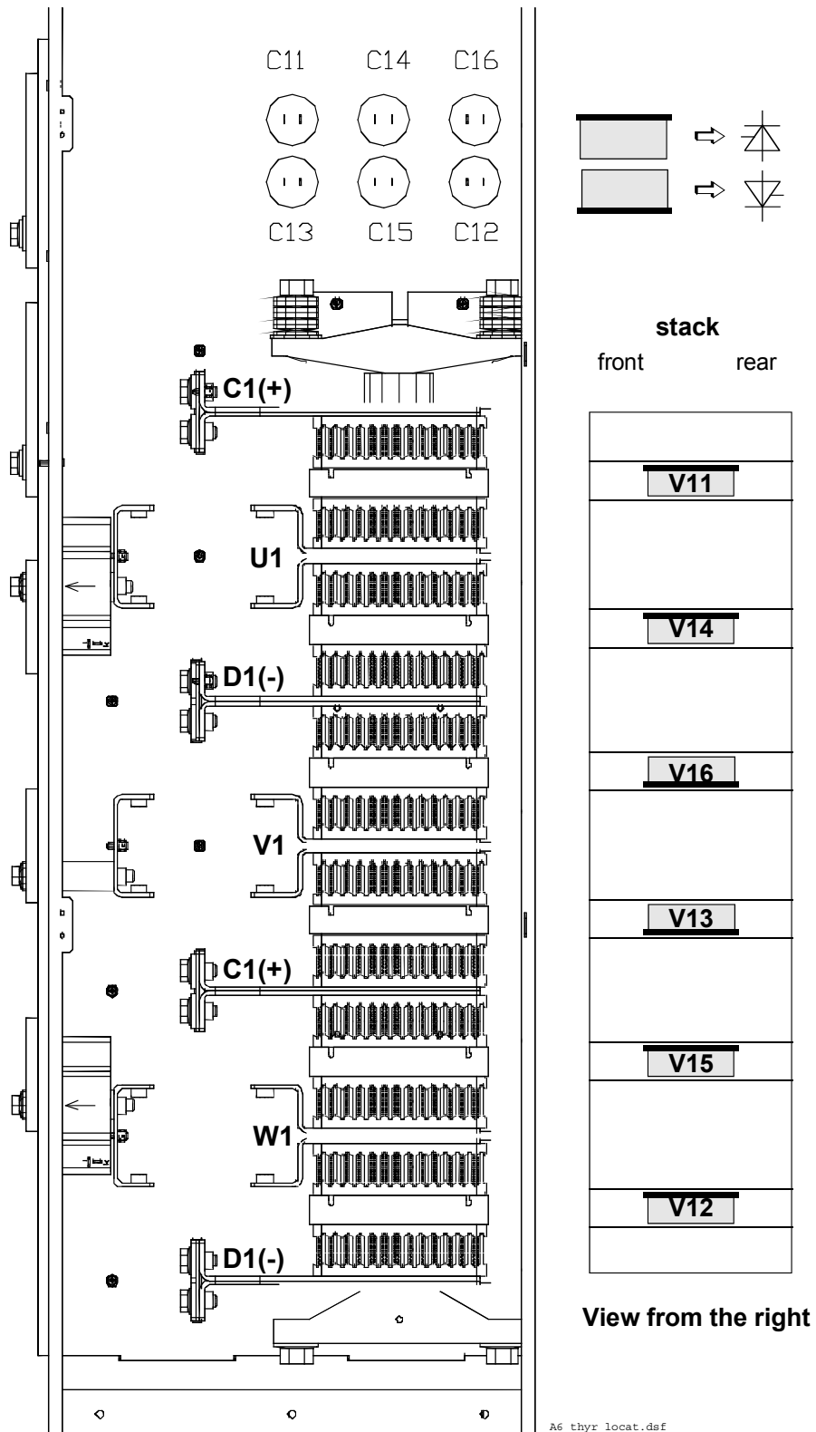
Location of thyristors in frame D6 (2-Q bridge with single thyristors)
