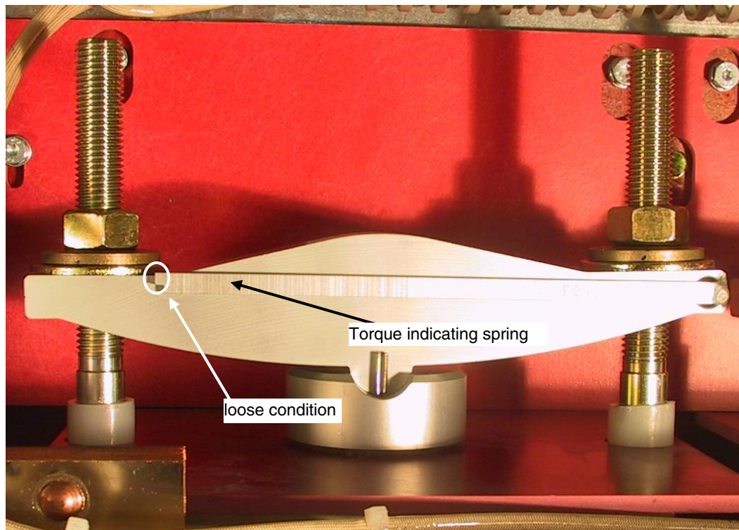
Mounting clamp; loose condition
