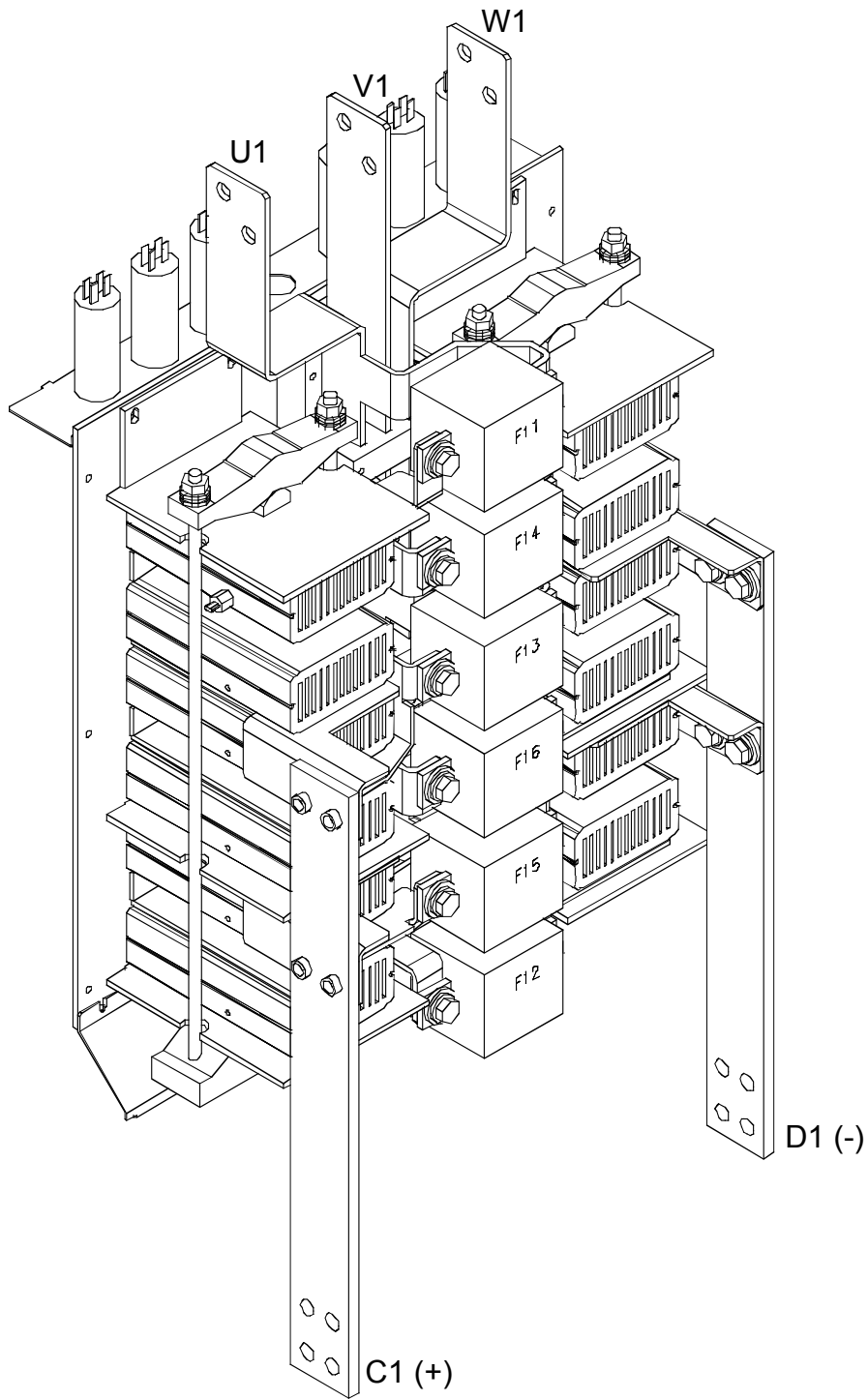
Location of branch fuses frame D5
