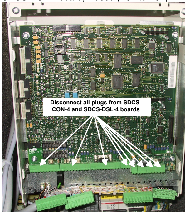
Disconnect all plugs
