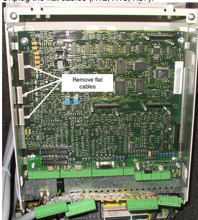
Unplug the flat cables
