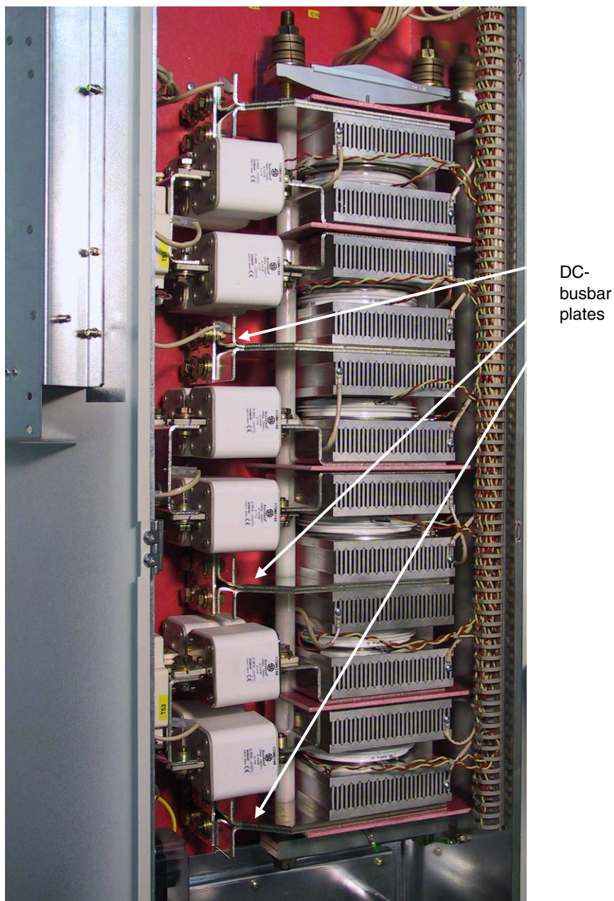
Location of the DC - busbar plates
