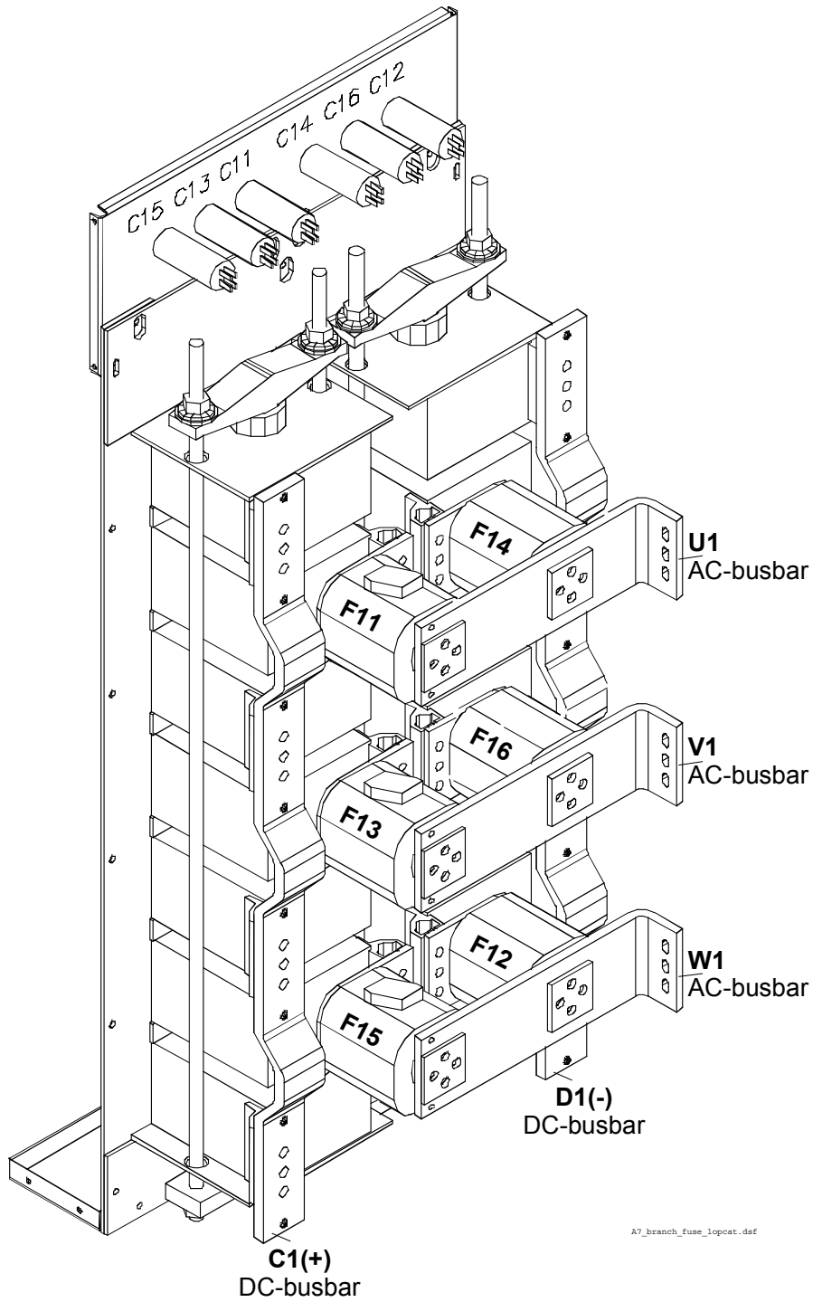
Location of branch fuses frame D7 (busbars on the right)
