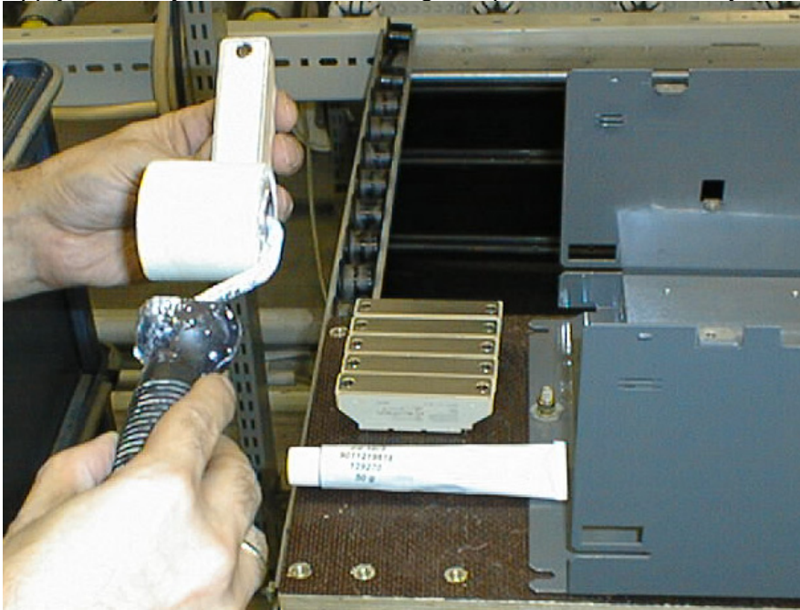
Application of heat conducting compound
