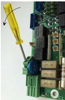
Remove cables at the SDCS-PIN-4
