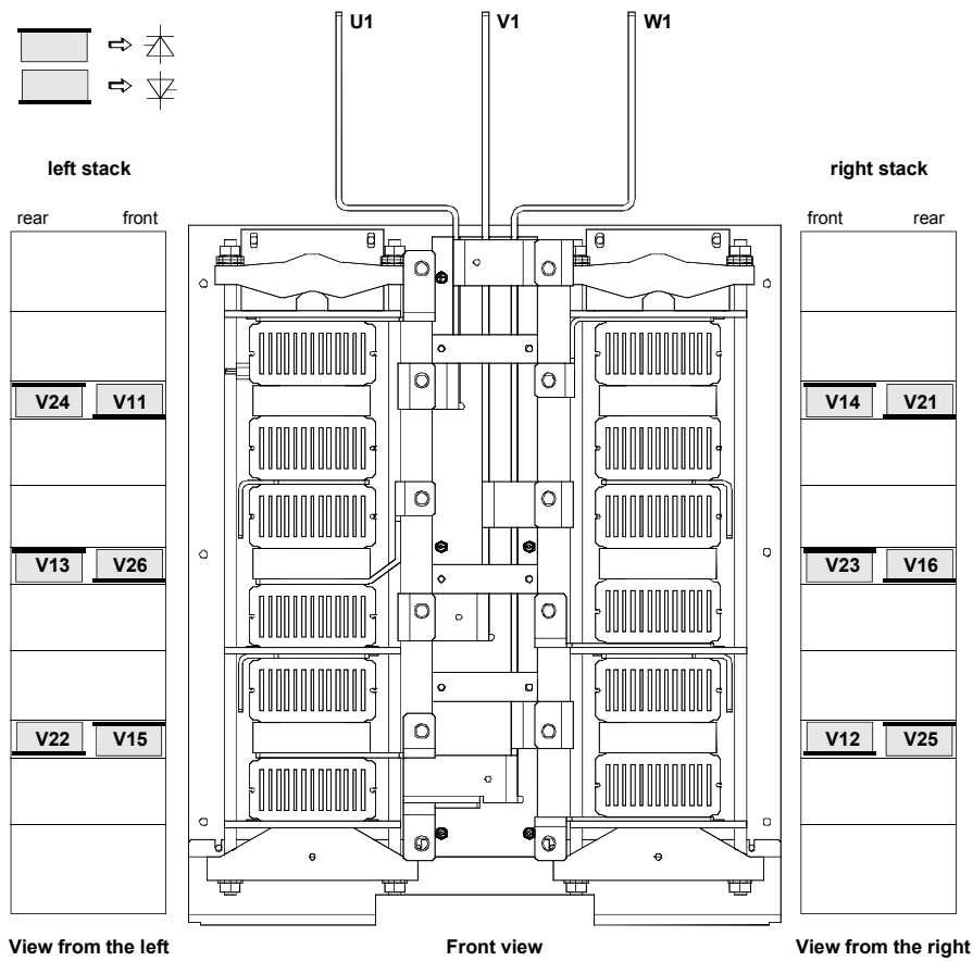
Location of thyristors in frame D5 (4-Q bridge)
