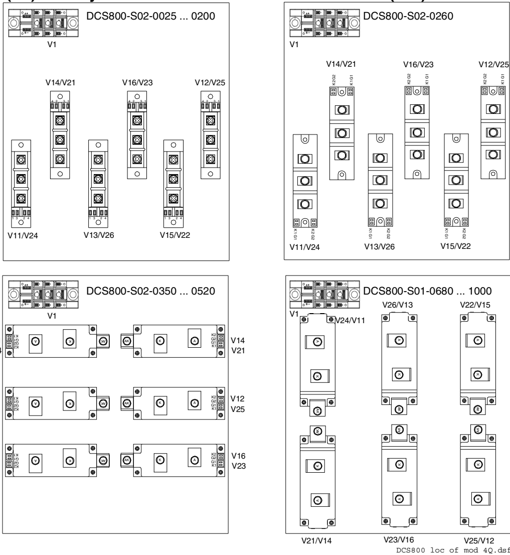
Location of the OnBoard bridge and thyristor modules in DCS800-S02 (4-Q) units
