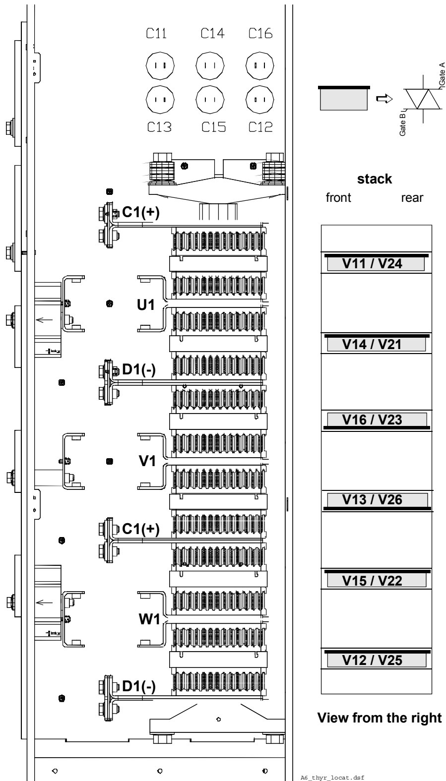
Location of thyristors in frame D6 (4-Q bridge with BCT's)
