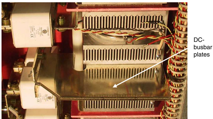
DC-busbar plates
