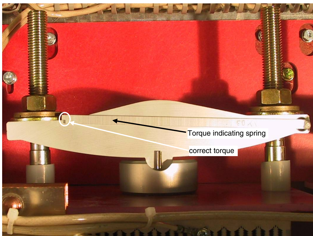
Mounting clamp; correct torque
