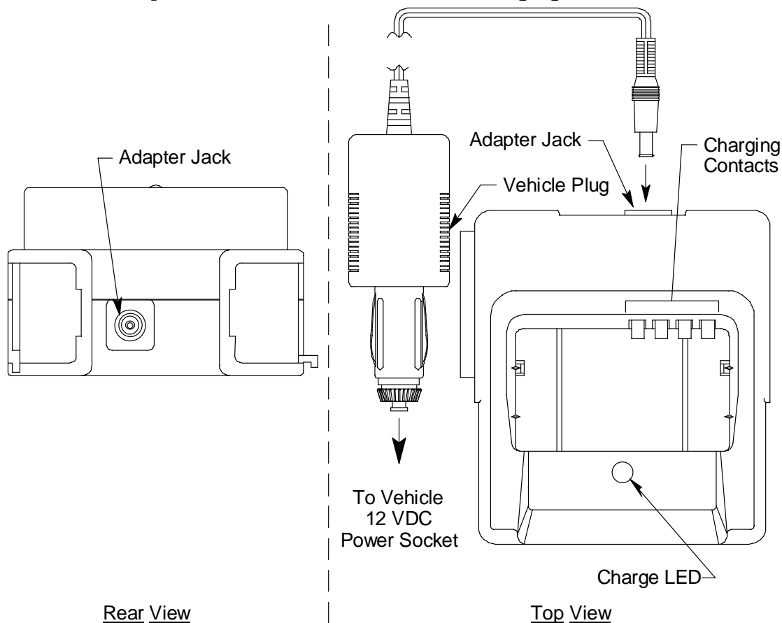
Figure 6: Gas Tracer DC Powered Charging Station
