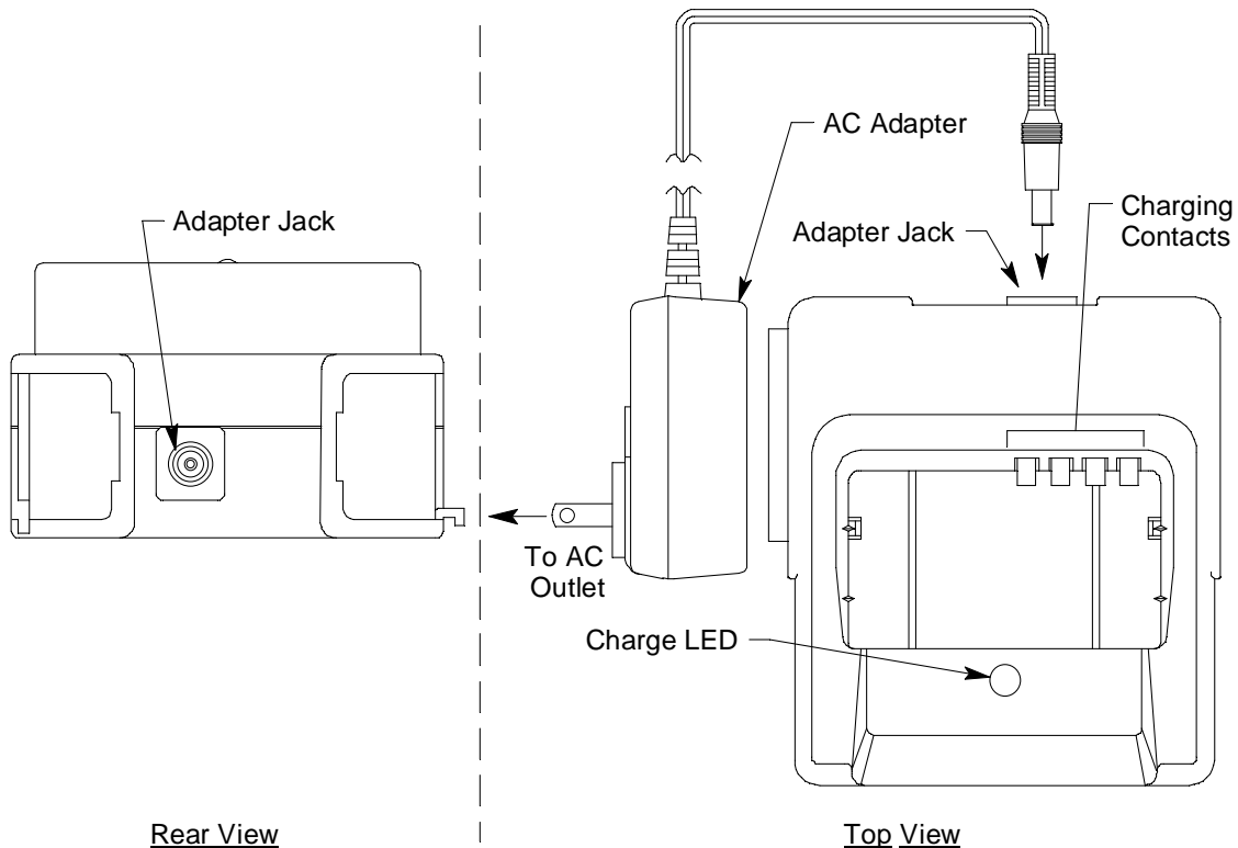
Figure 5: Gas Tracer AC Powered Charging Station
