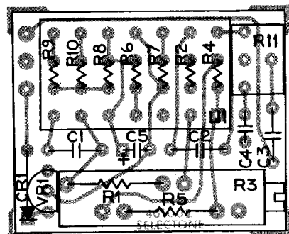
SOLDER SIDE
