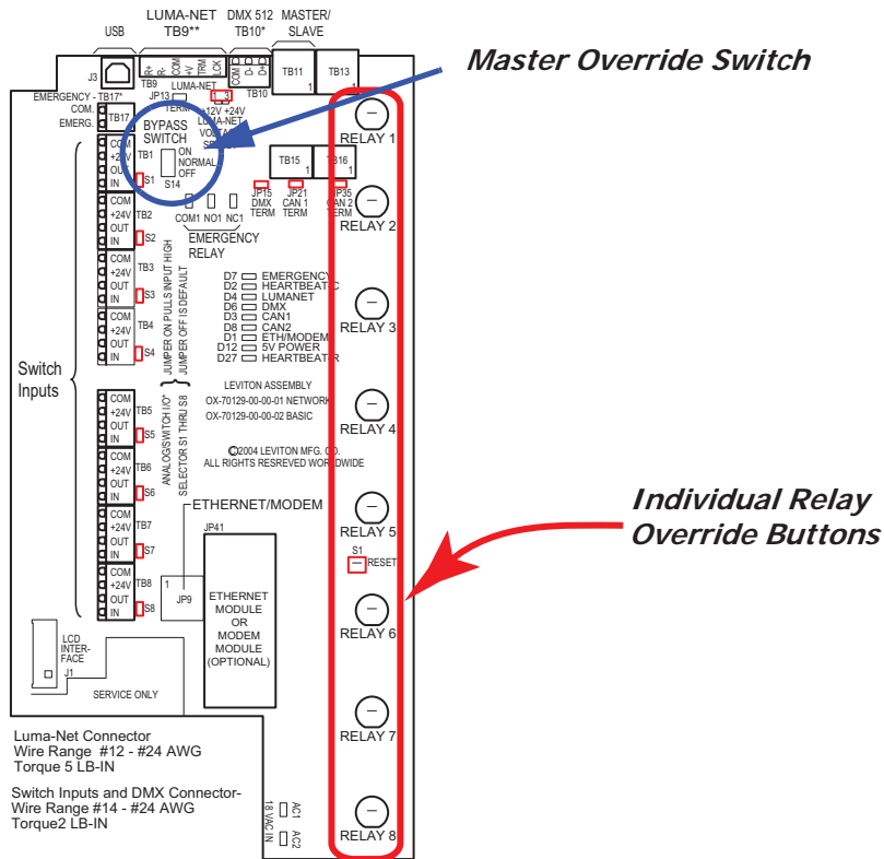
Figure 7: Location of Individual Relay Override Buttons in the 8 Cabinet
