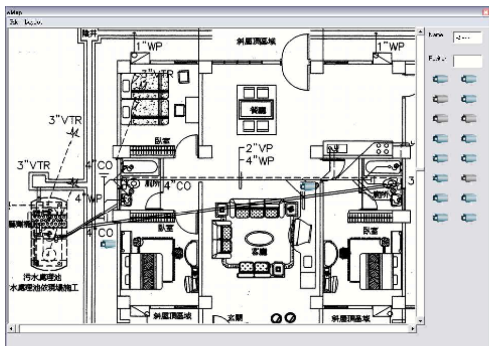
Figure 5.8.2. Layout example 2
