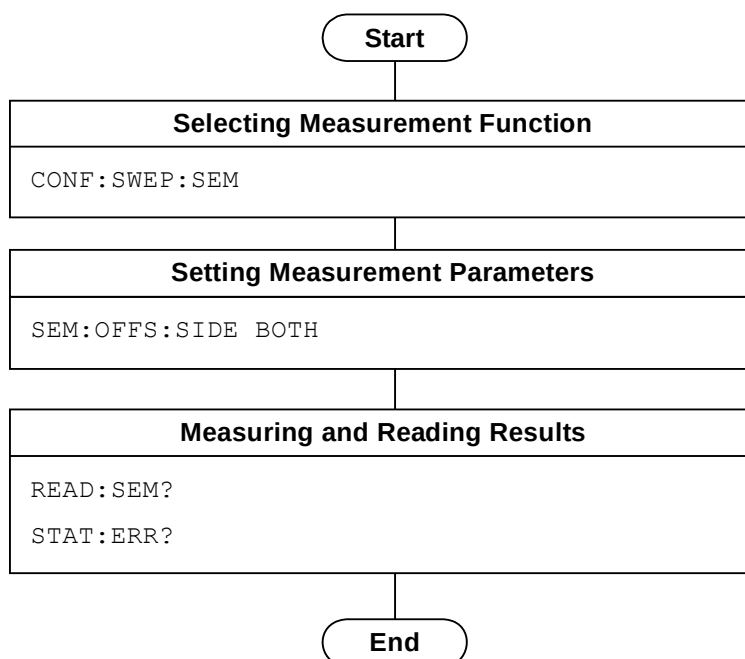
Figure 1.2.10-1 Flow of SEM Measurement using Spectrum Analyzer and Command Example
