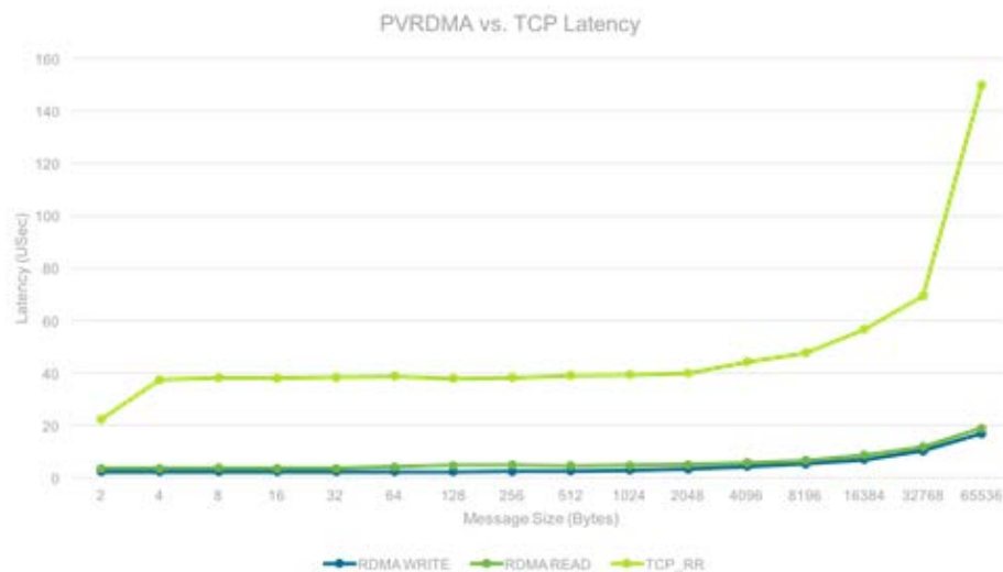
Figure 10. RDMA write and read show lower latencies than that of TCP
