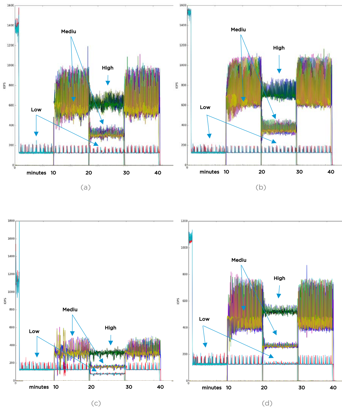
Figure 6. Performance impact of using SIOC in datacenter: (a) sequential write, (b) sequential read, (c) random write, and (d) random read
