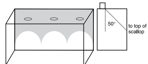
Scallops placed too low on wall will cause a "cave effect"
