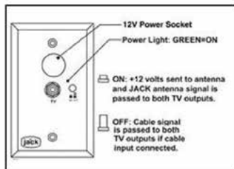
Power Injector
