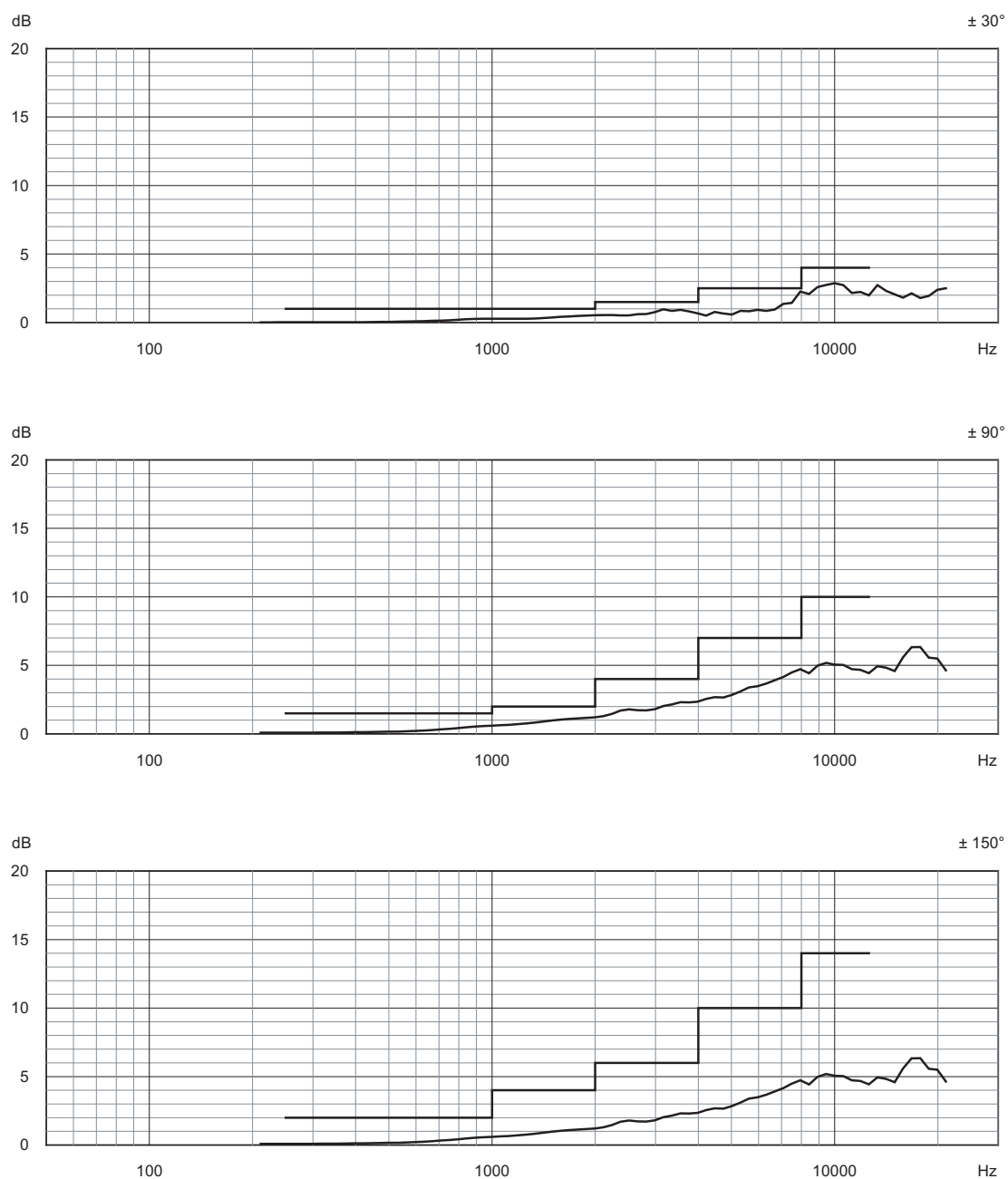
Fig. 4.18b 4952 90° (Side), sensitivity variations for Outdoor Microphone Type 4952 with the Microphone Preamplifier connected to a microphone extension cable, at sound incidence angles within \pm\theta^\circ from the reference direction. Corresponds to Table A.34b
