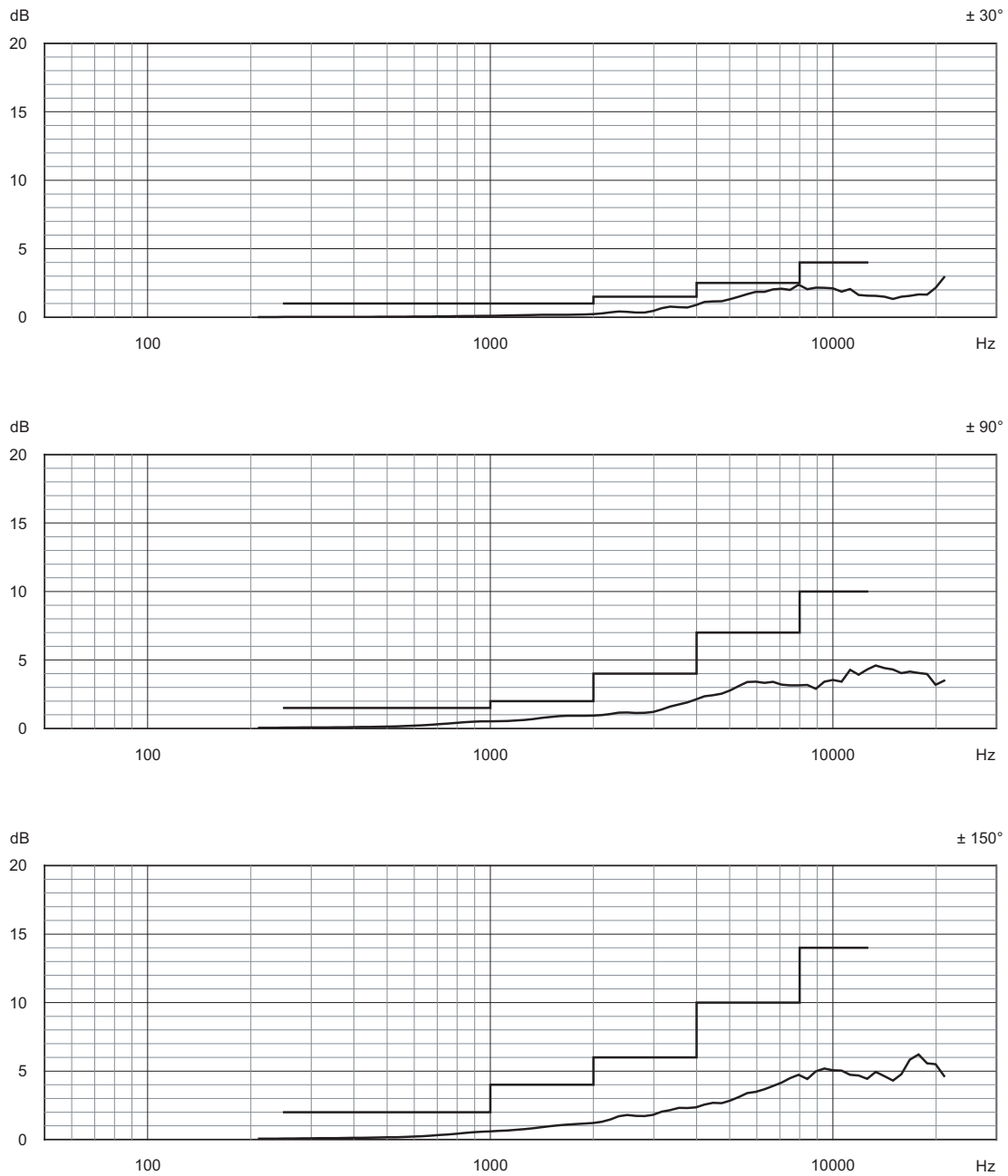
Fig.4.18a 4952 0° (Top), sensitivity variations for Outdoor Microphone Type 4952 with the Microphone Preamplifier connected to a microphone extension cable, at sound incidence angles within \pm\theta^\circ from the reference direction. Corresponds to Table A.34a
