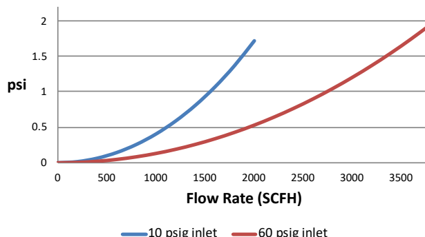
Pressure Drop
