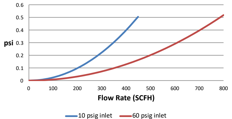
Pressure Drop
