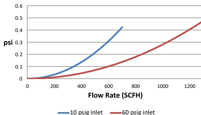
Pressure Drop
