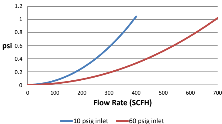
Pressure Drop
