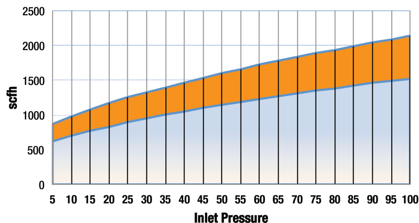
Pressure Drop
