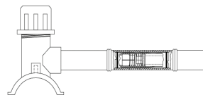
Model 70 — Tee with Model 41 attached
