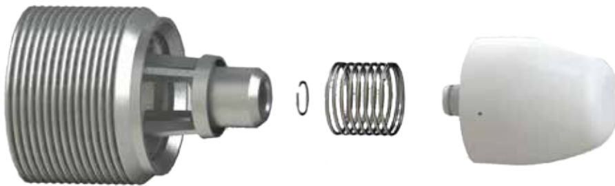
Nozzle/Valve Seat
