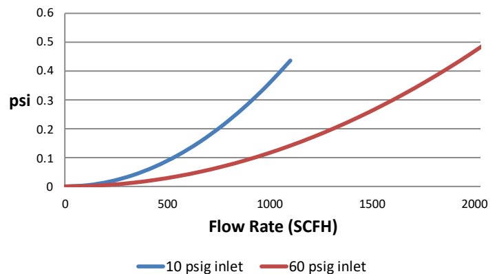
Pressure Drop
