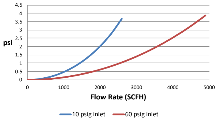
Pressure Drop
