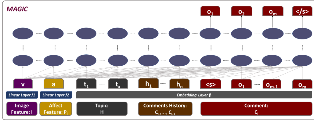
Figure 5: Overview of MAGIC model architecture
