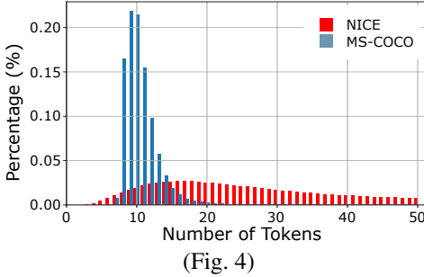
Figure 4: Histogram of the length of sentences in NICE dataset and COCO dataset.
