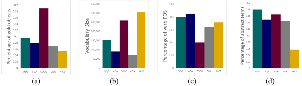
Figure 3: Comparison of annotations on the NICE dataset: (a) % of human-labeled objects used in annotations, (b) vocabulary size, (c) % of verb POS, (d) % of abstract terms.
