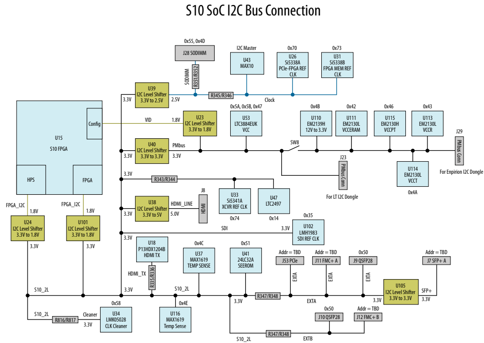
Figure 28. HPS I 2 C Interface
