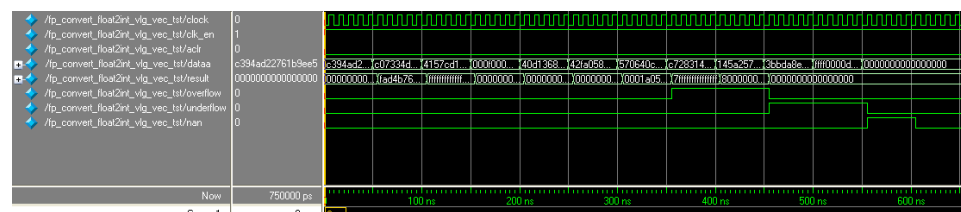
Figure 39. ALTFP_CONVERT Simulation Waveform
