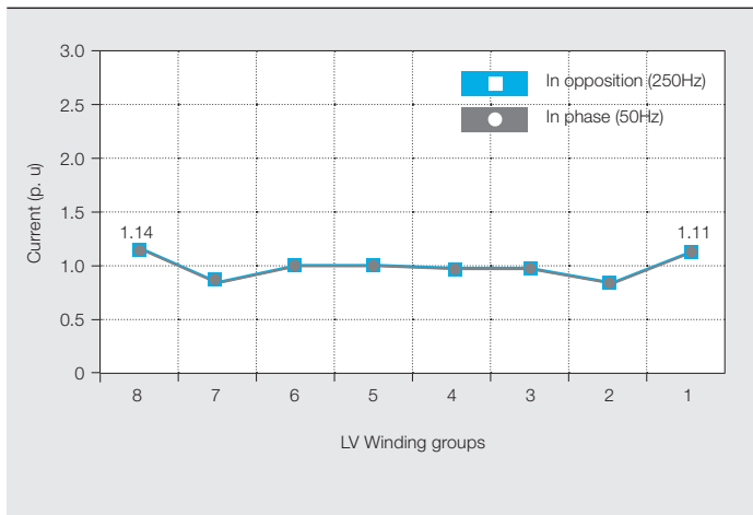
3c Upper tier C1 with intermediate yoke
