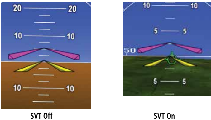
Figure 5-36 Flight Director Bars Showing Aircraft Pitch
