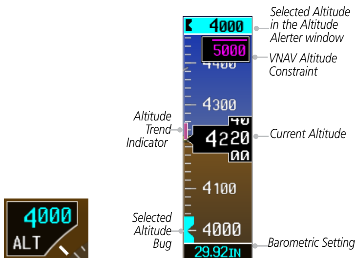
Figure 2-21 Altimeter
