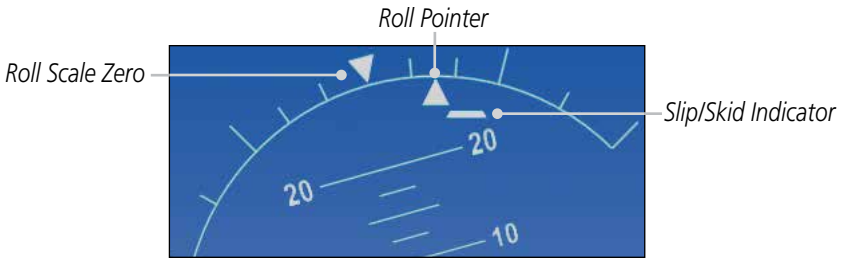
Figure 2-15 Slip/Skid Indication
