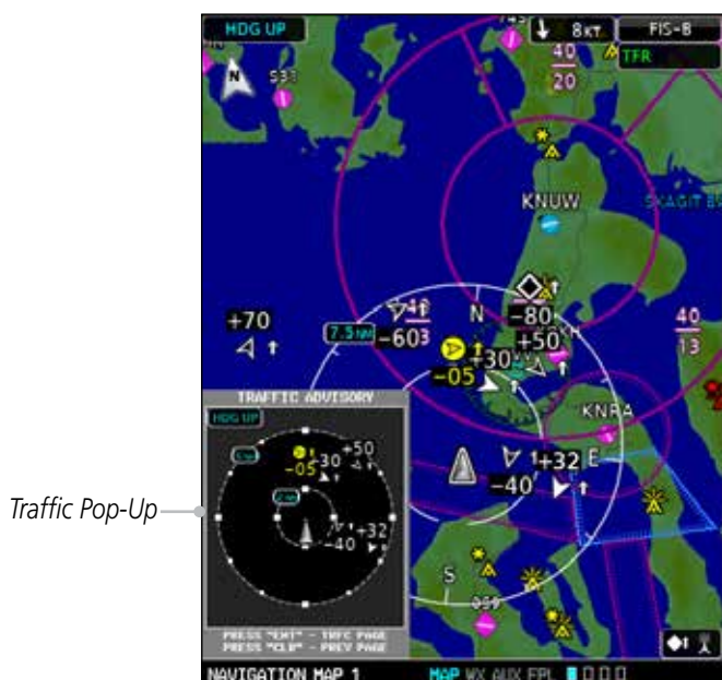
Figure 4-28 Traffic Pop-Up
