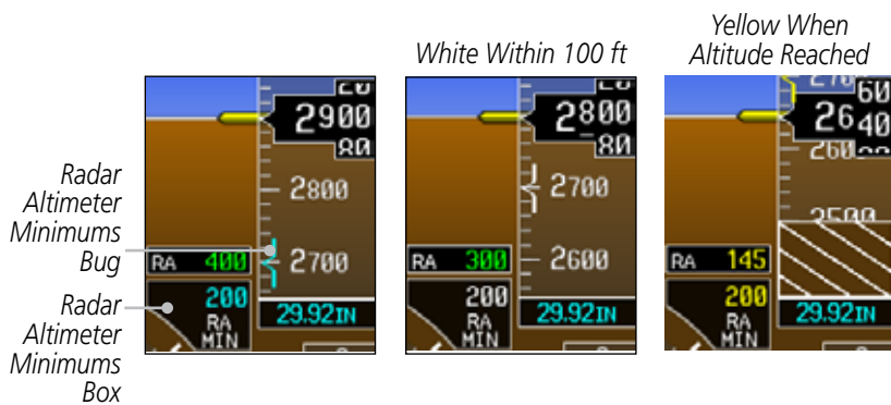
Figure 2-25 Radar Altimeter - Alerting Visual Annunciations
