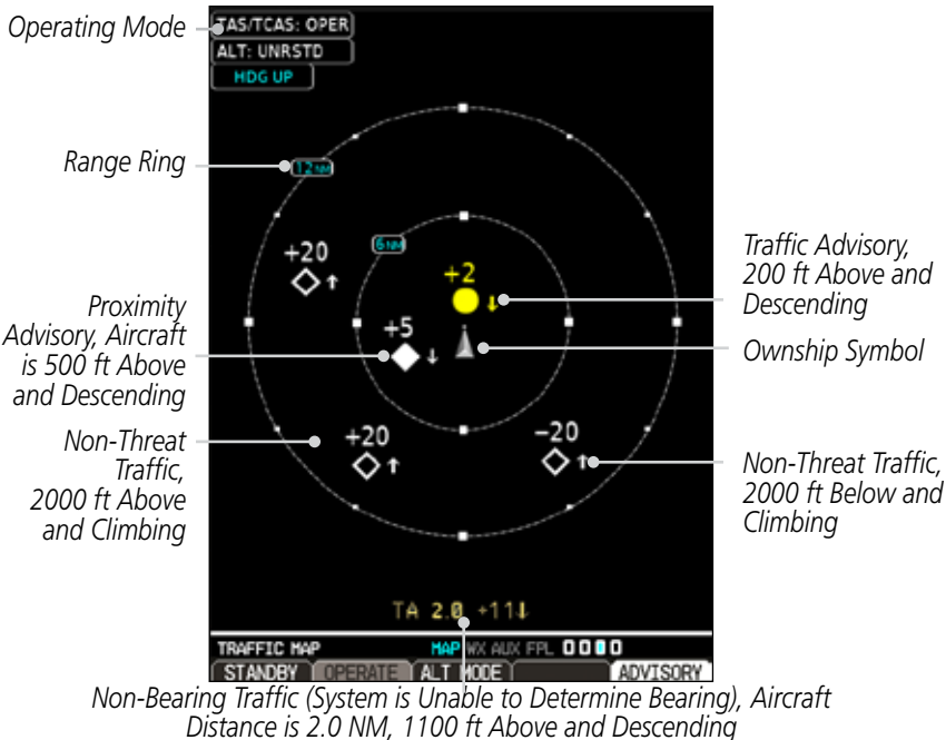
Figure 4-29 Traffic Map Page - TAS/TCAS
