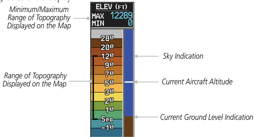
Figure 3-18 Navigation Map Topo Scale
