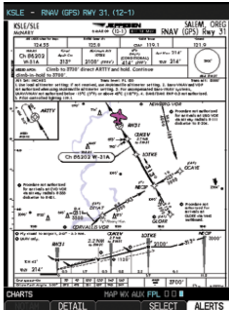
Figure 5-10 Selected Chart for the Current Airport (ChartView)
