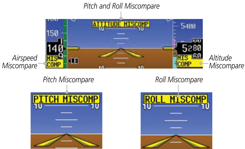
Figure 2-47 Mismatch Annunciations
