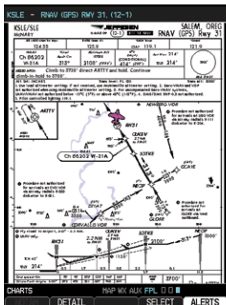
Figure 5-12 Selected Chart for the Current Airport (ChartView)
