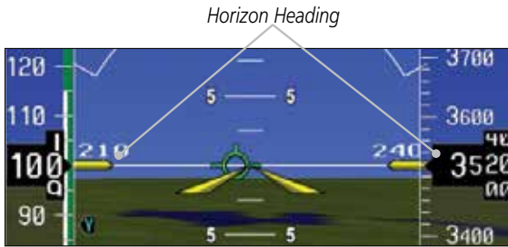
Figure 5-45 Horizon Heading
