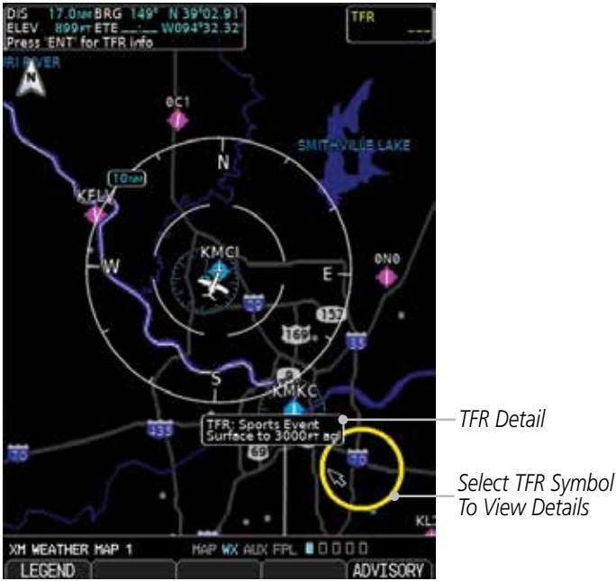
Figure 4-59 XM Weather - TFRs
