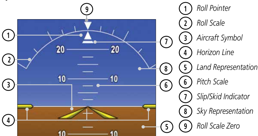
Figure 2-14 Attitude Indicator
