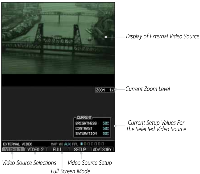
Figure 3-64 External Video
