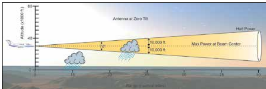
Figure 4-71 Radar Beam from 12 inch Antenna
