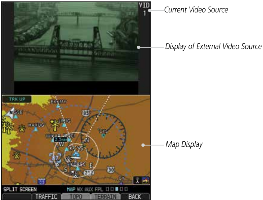
Figure 3-34 External Video
