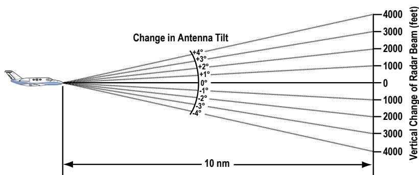
Figure 4-76 Vertical Change in Radar Beam per Nautical Mile
