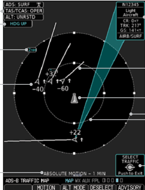
Figure 4-32 ADS-B Traffic Page (Absolute Motion)
