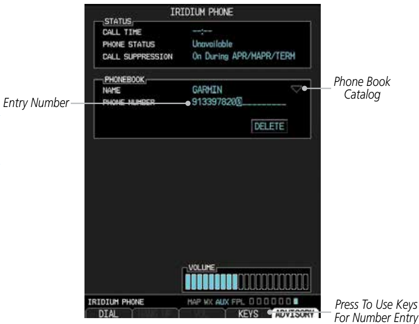
Figure 3-80 Phone Book Number Entry
