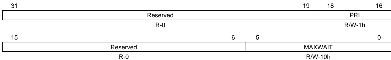
Figure 6-1. CPU Arbitration Control Register (CPUARB, CPUARBU, CPUARBE)
