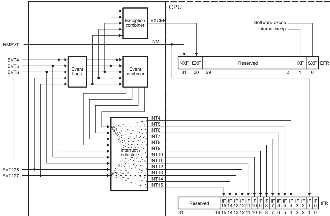
Figure 7-14. CPU Event Routing Diagram
