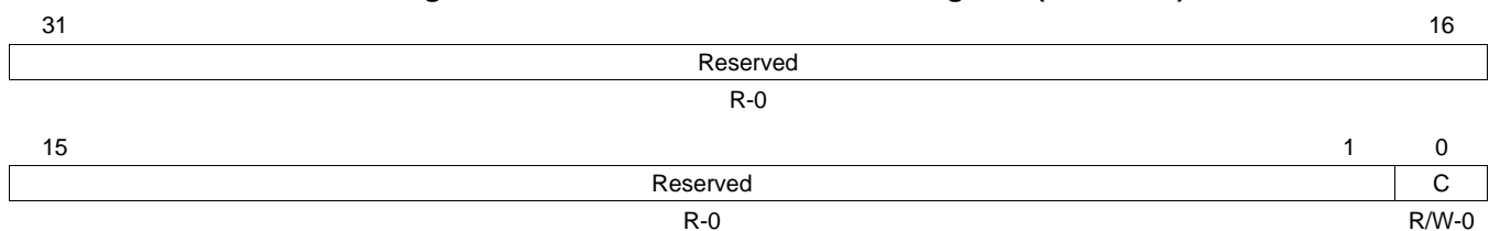
Figure 4-10. L2 Writeback-Invalidate Register (L2WBINV)
