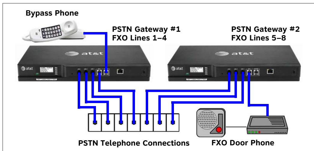
Figure 9. Trunk Port (FXO) Door Phone Connection
