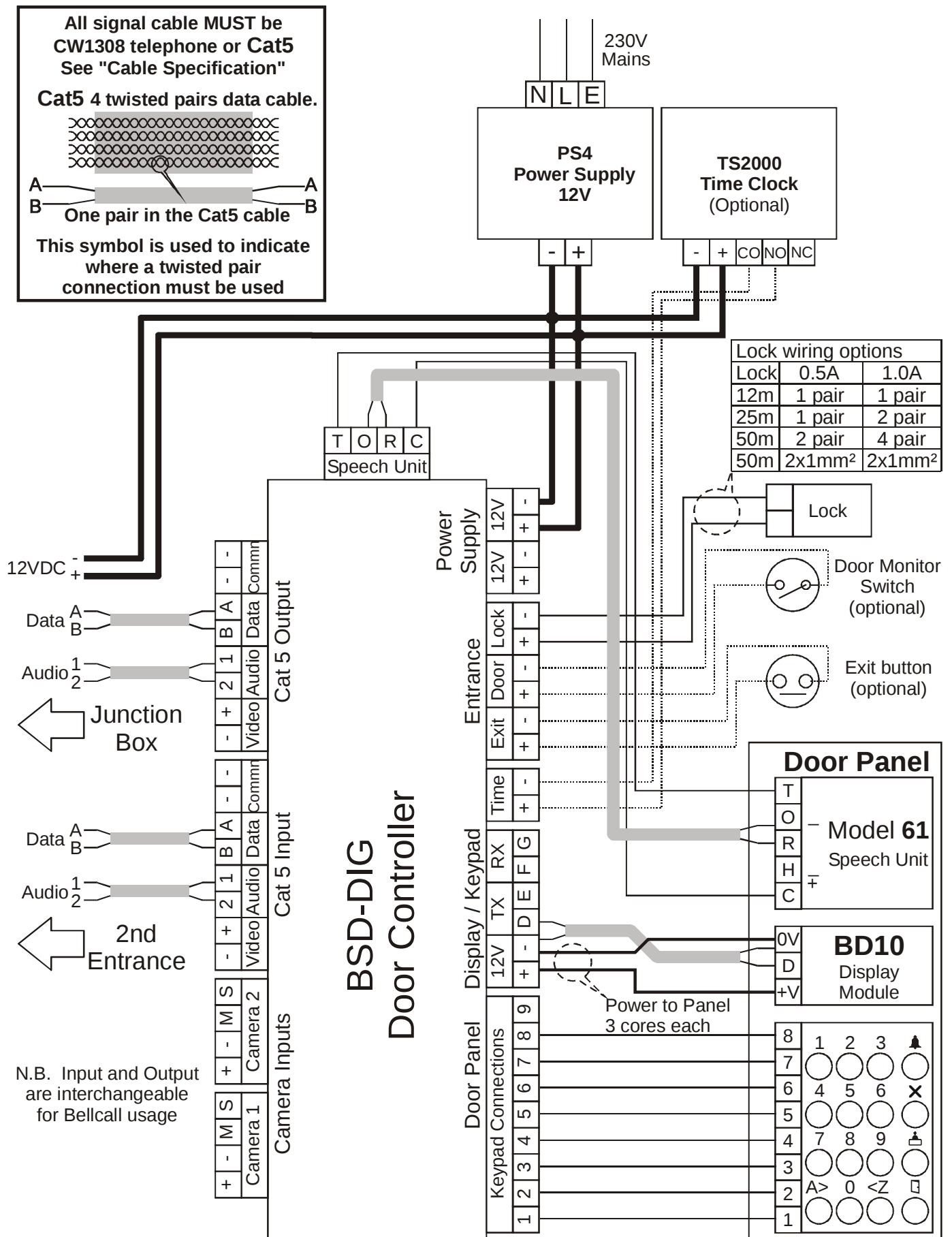
Diagram H – BSD-DIG VR or LCP Panel Detail Wiring
