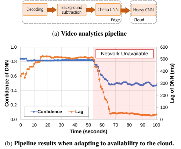
Figure 2: Network adaptation for video analytics.
