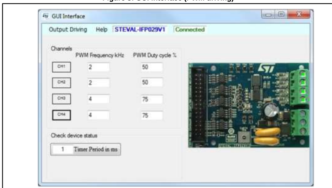
Figure 8: GUI interface (PWM driving)
