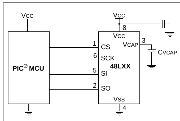
FIGURE 2: TYPICAL SPI APPLICATION
