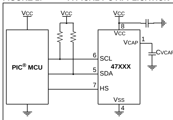
FIGURE 1: TYPICAL I 2 C APPLICATION
