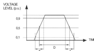
Figure 1: Test waveform
