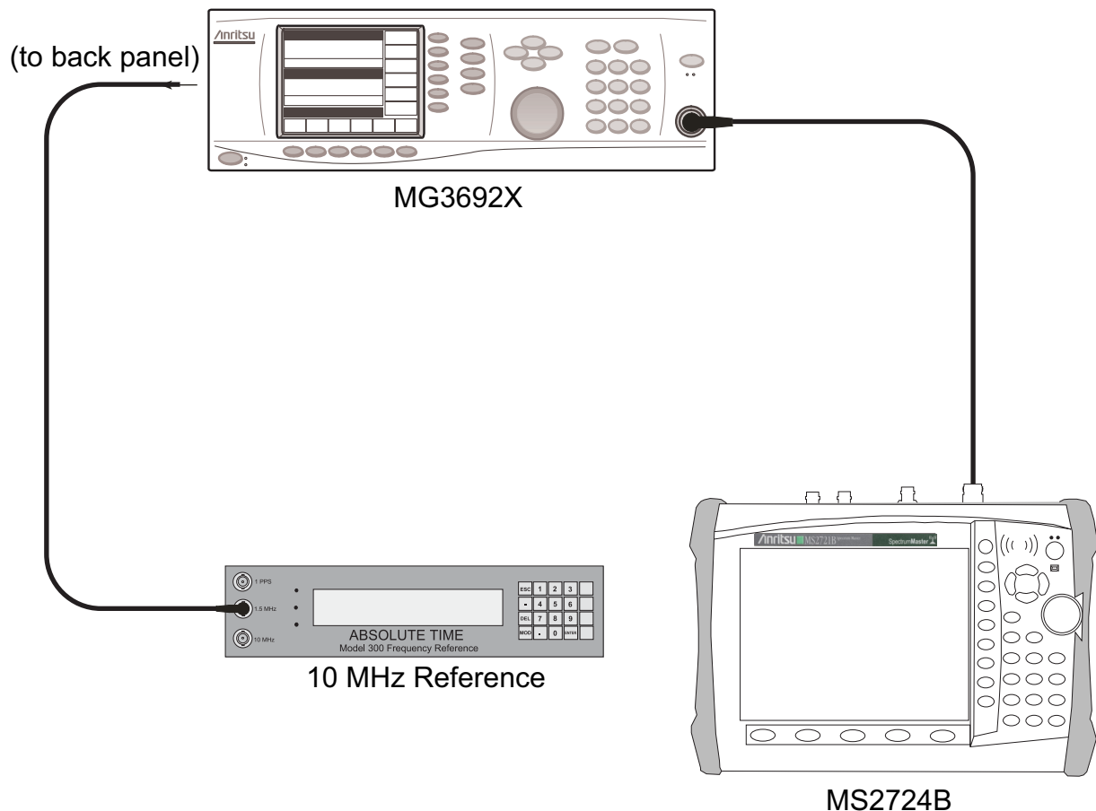
Figure 2-8. Input Related Spurious Signals – Test Setup
