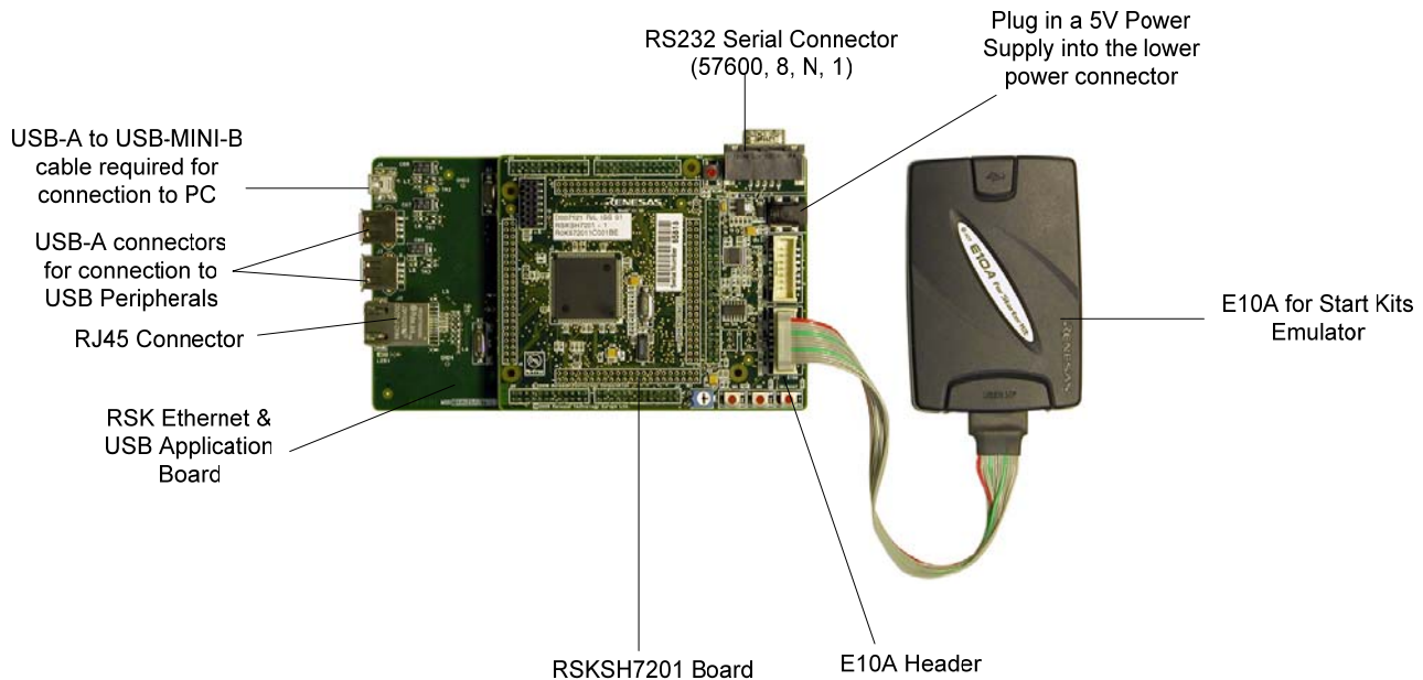
Fig 2.1 Connections to the system
