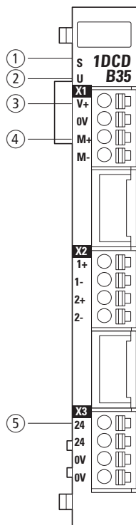
Figure 122: XN-322-1DCD-B35 LEDs
