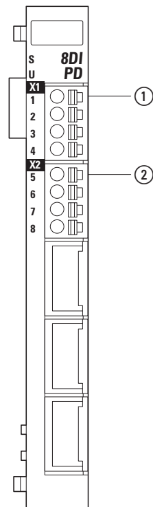
Figure 24: Pin assignment
