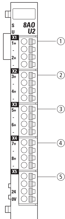
Figure 95: Pin assignment
