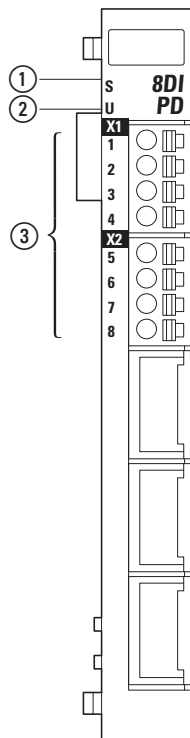
Figure 23: LED signals and pin assignment for XN-322-8DI-PD
