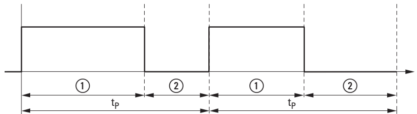
Figure 73: PWM signal measurement
