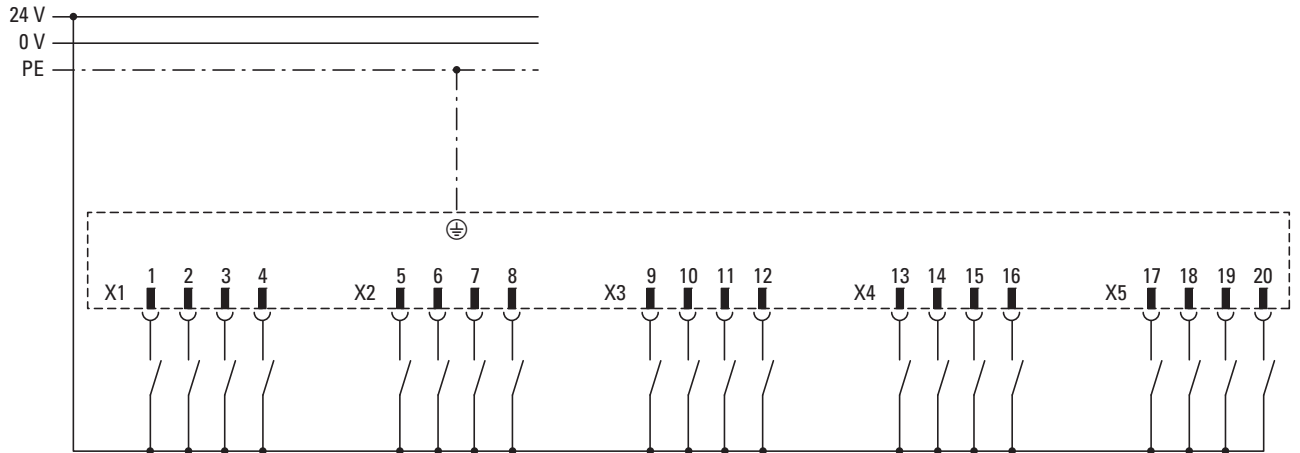
Figure 34: Input wiring
