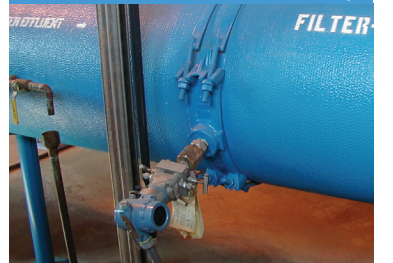
485 Annubar air flow to aeration
