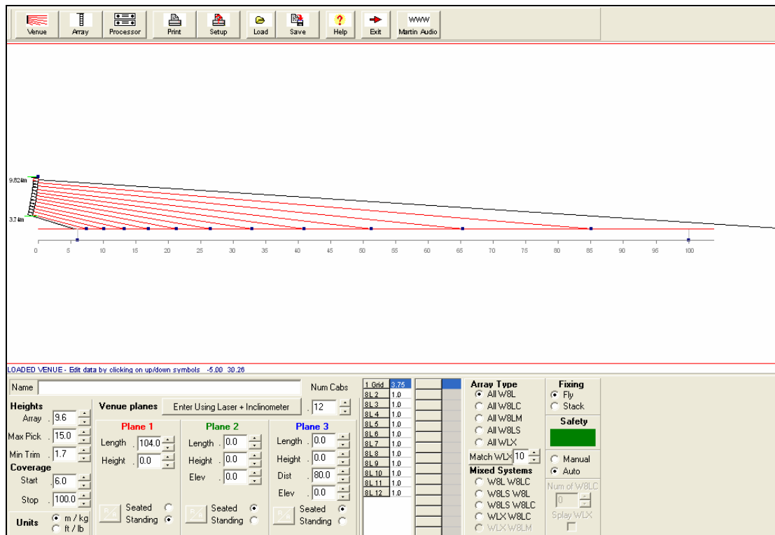
12 x W8L (at 1°) per side festival system in side wings for 100m throw
