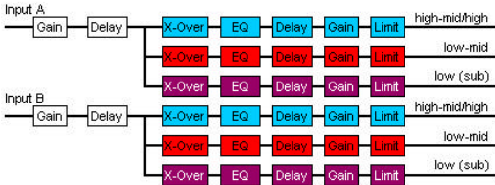
DX1 factory preset 20 (2 x 3 way configuration) Stereo W8 system (passive) with WSX subwoofers
