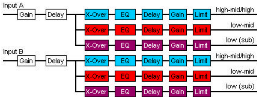
DX1 factory preset 20 (2 x 3 way configuration) Stereo WSX+W8C (passive high-mid/high) system
