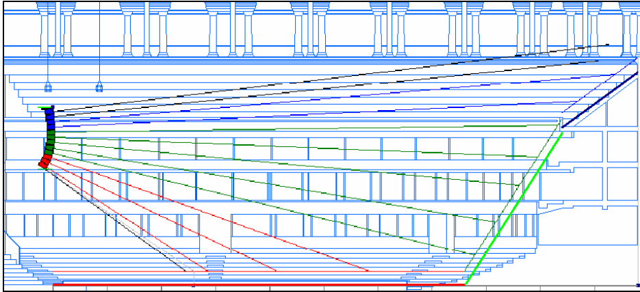
Overlaid ViewPoint™ display (front fills not shown)
