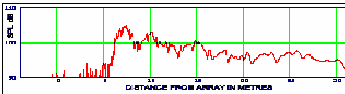
Smoother coverage from a Martin Audio Progressive Curvature Array
