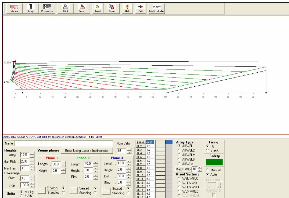
16 x W8L per side arena system Upper 12 cabinets at 1 & 2° for 100m throw
