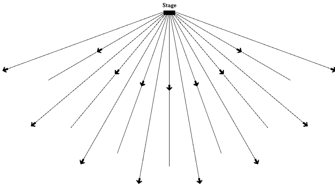
Distributed flown loudspeaker plan (stage system not shown)
