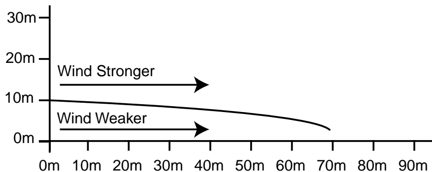
Sound path tilting downwards outdoors due to wind blowing away from loudspeakers
