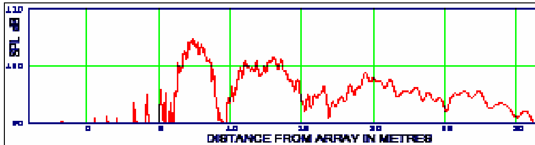
Irregular coverage from a J-Shaped Array
