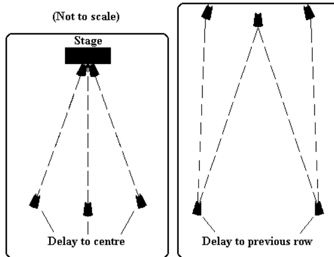
Synchronising flown central delays
