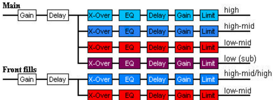
3 + 2-way configuration e.g. W8 3-way system with W8S subs (passive) & W8 (passive) front fills
