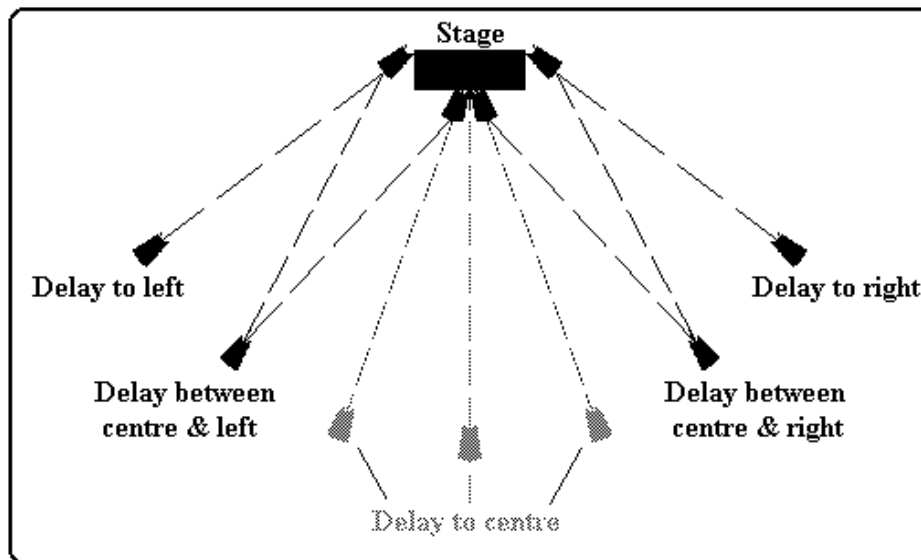
Synchronising flown outer delays
