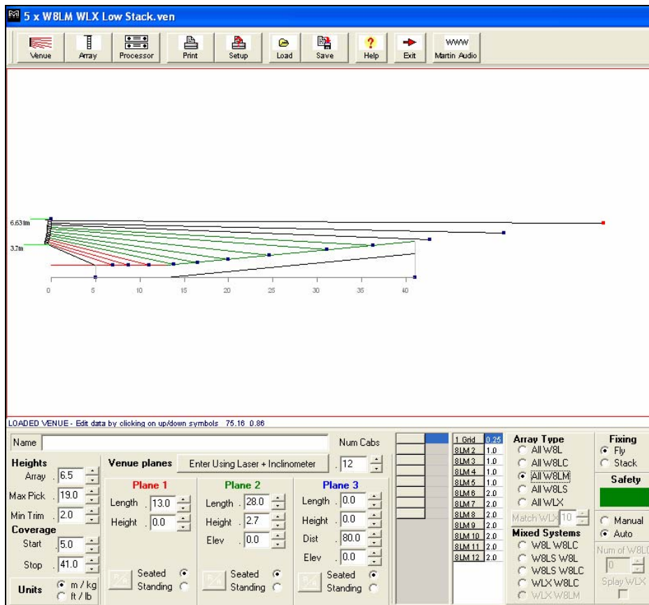
12 x W8LM per side 41m concert hall system
