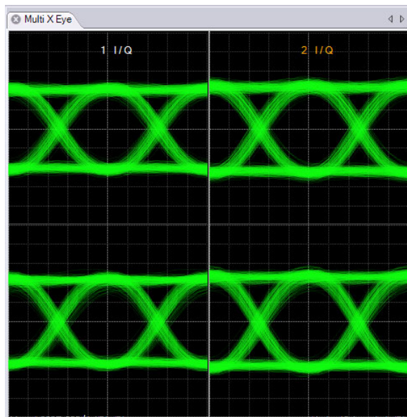
Figure 11: Multicarrier Eye diagrams plot
