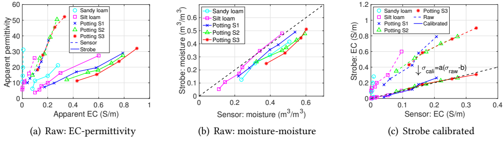
Figure 11: Soil permittivity and EC estimation with Strobe and Decagon GS3 sensor. Strobe calibration: EC is calibrated based on ground truth EC measured by the soil sensor. Salinity level: S3>S2>S1.
