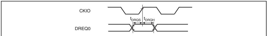
Figure 52.39 DREQ Input Timing
