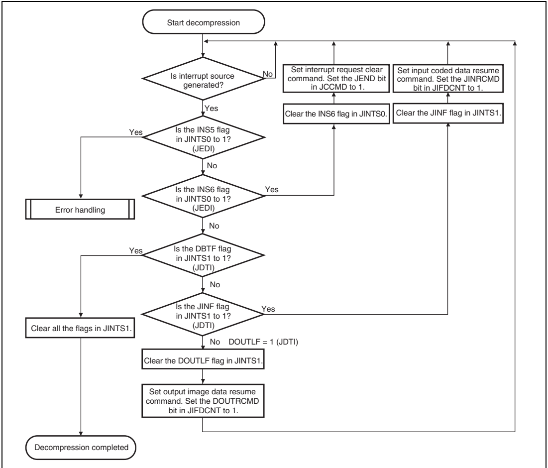
Figure 41.9 Decompression Process Flow
