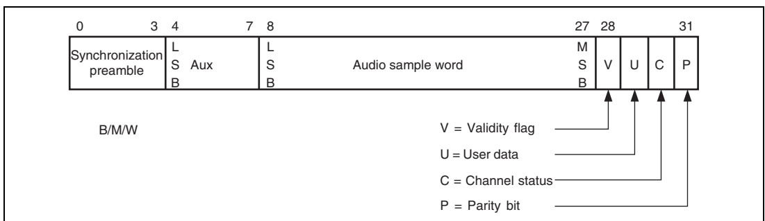
Figure 25.3 Subframe Format
