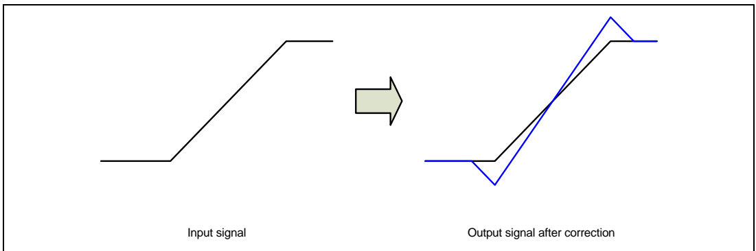
Figure 34.6 Sharpness Correction
