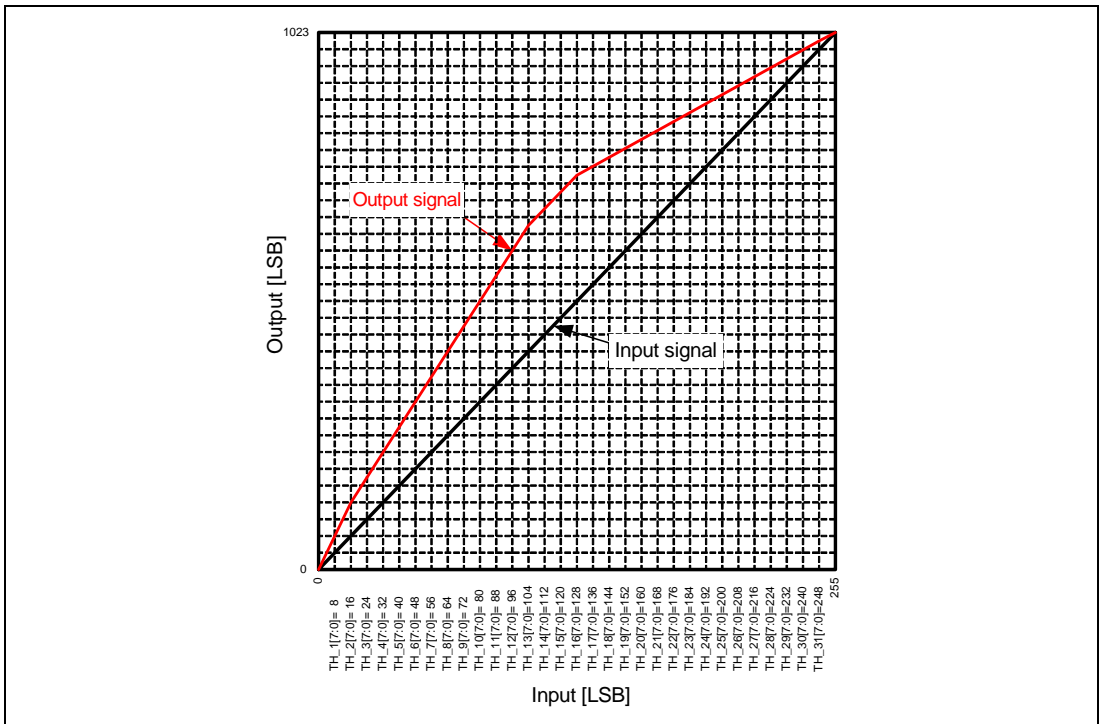
Figure 36.3 Example of Input-Output Characteristics of Gamma Correction
