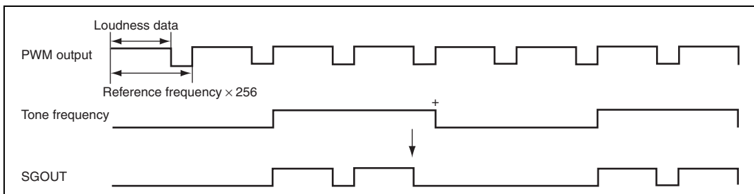
Figure 43.5 Output Waveforms
