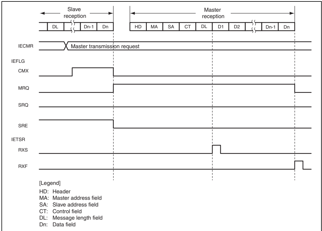
Figure 24.15 Master Receive Operation Timing
