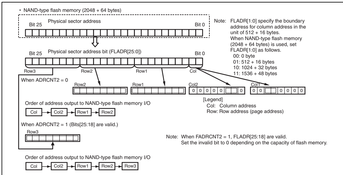
Figure 28.11 Relationship between Sector Number and Address Expansion of NAND-Type Flash Memory
