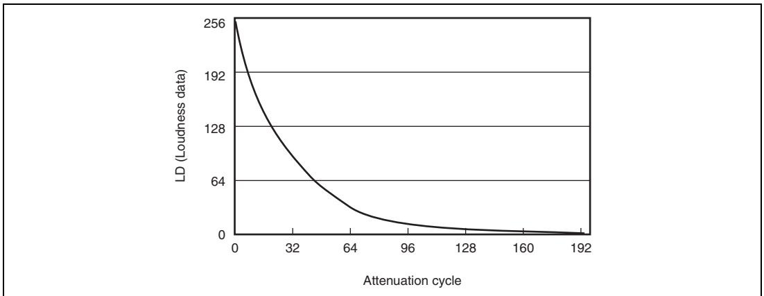
Figure 43.4 Attenuation Characteristics
