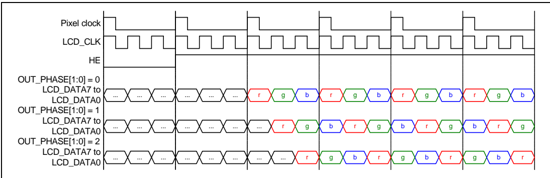
Figure 36.7 Timing of Clock Phases of Serial RGB Output (Triple Speed Mode)
