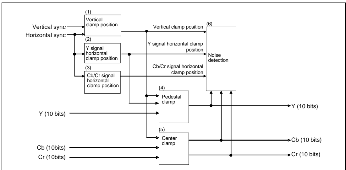
Figure 30.37 Block Diagram of Digital Clamp Circuit
