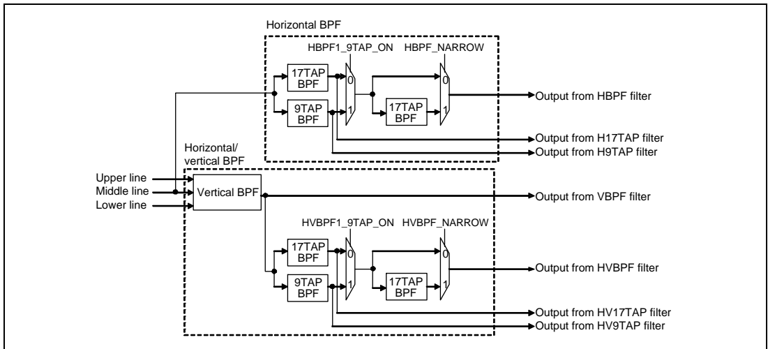
Figure 30.32 Horizontal and Vertical Filter Configuration
