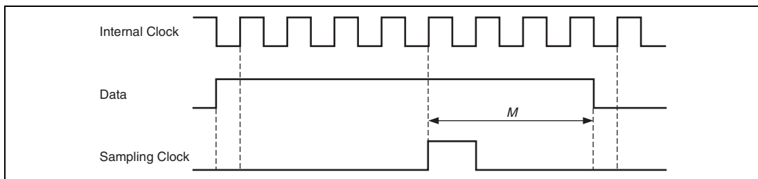
Figure 25.7 Receive Margin
