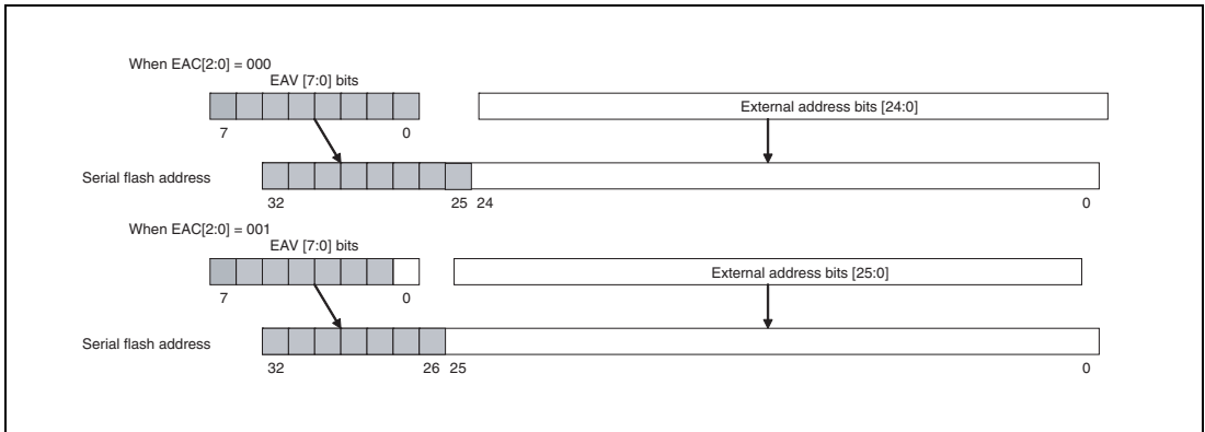
Figure 19.4 32-Bit Address Setting
