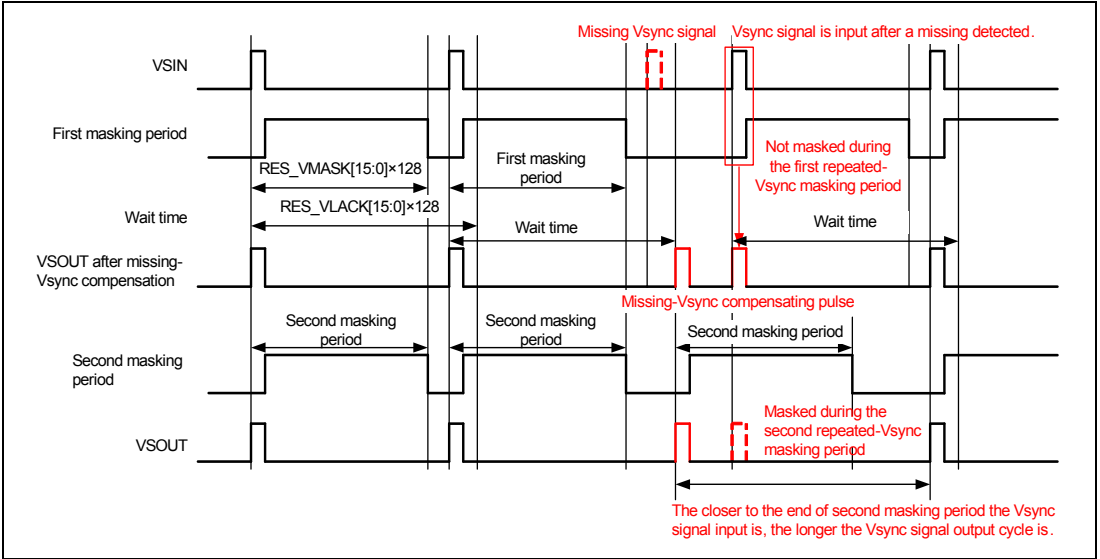
Figure 33.5 Timing for Masking Repeated Vsync Signals and Missing Vsync Signal Compensation
