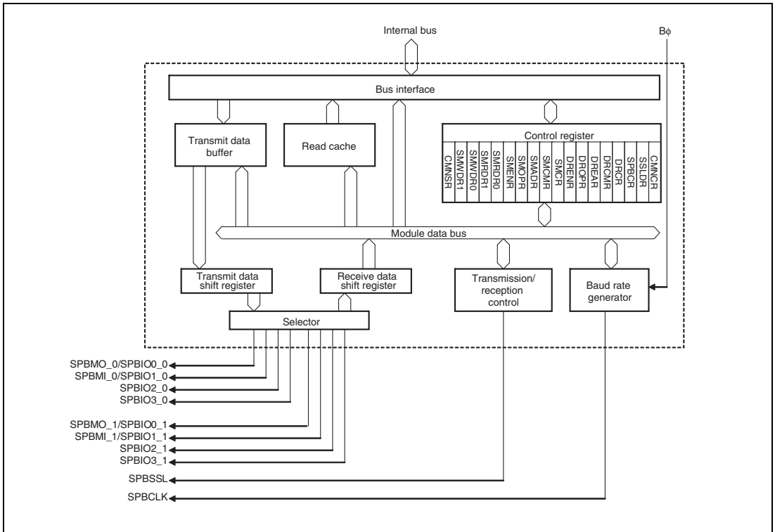
Figure 19.1 Block Diagram
