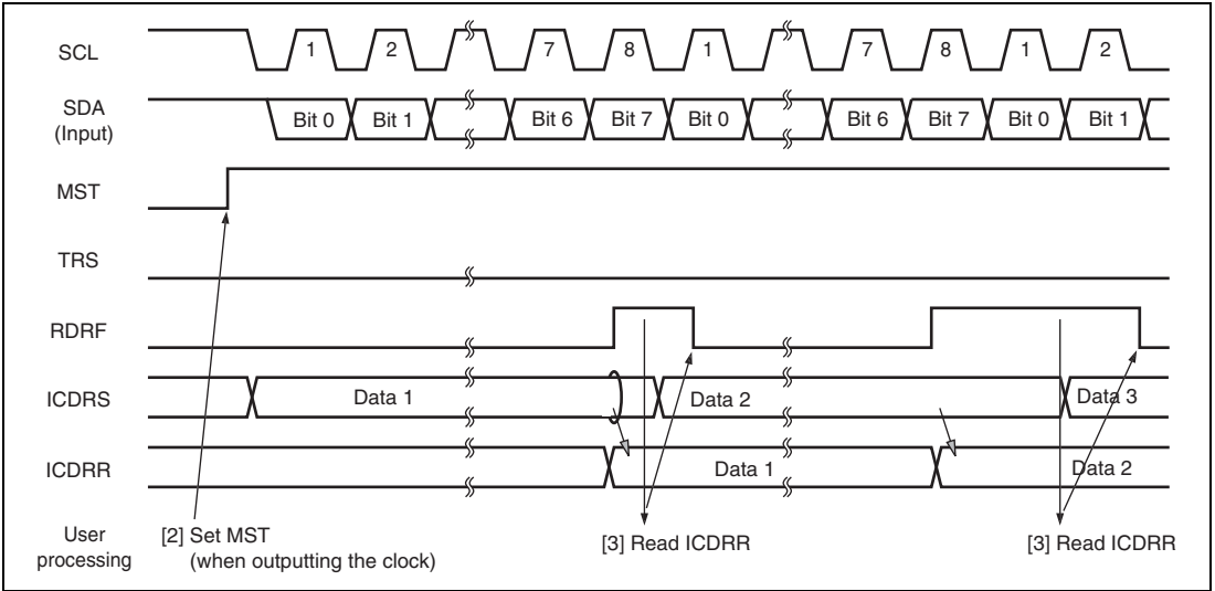
Figure 20.15 Receive Mode Operation Timing
