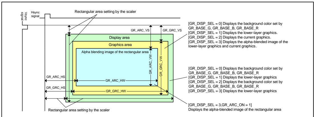
Figure 35.8 Graphic Display Types
