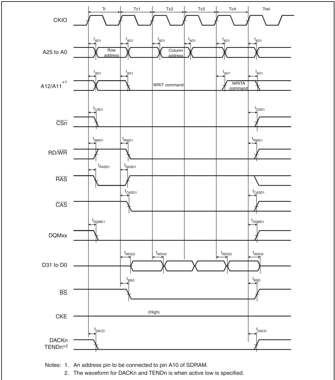
Figure 52.23 Synchronous DRAM Burst Write Bus Cycle (Four Write Cycles) (Auto Precharge, WTRCD = 0 Cycle, TRWL = 1 Cycle)
