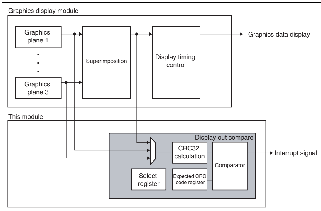
Figure 39.2 System Configuration
