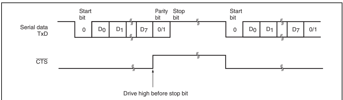
Figure 16.6 Example of Operation Using Modem Control ( \overline{CTS} )
