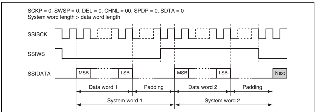
Figure 21.3 I 2 S Compatible Format (with Padding)
