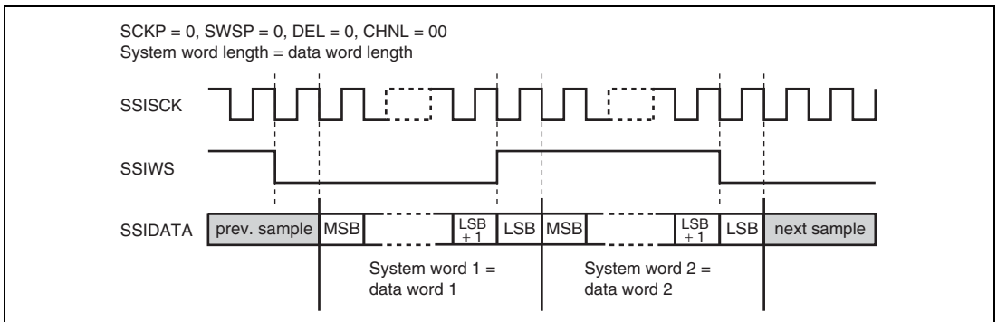
Figure 21.2 I 2 S Compatible Format (without Padding)
