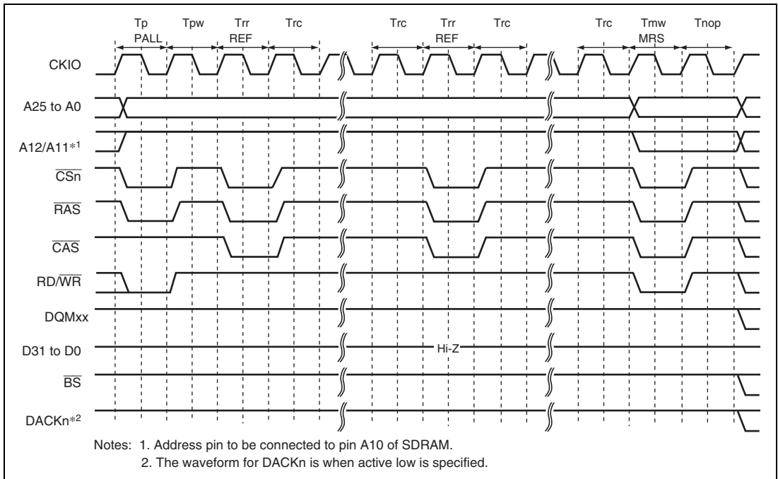
Figure 10.30 SDRAM Mode Write Timing (Based on JEDEC)
