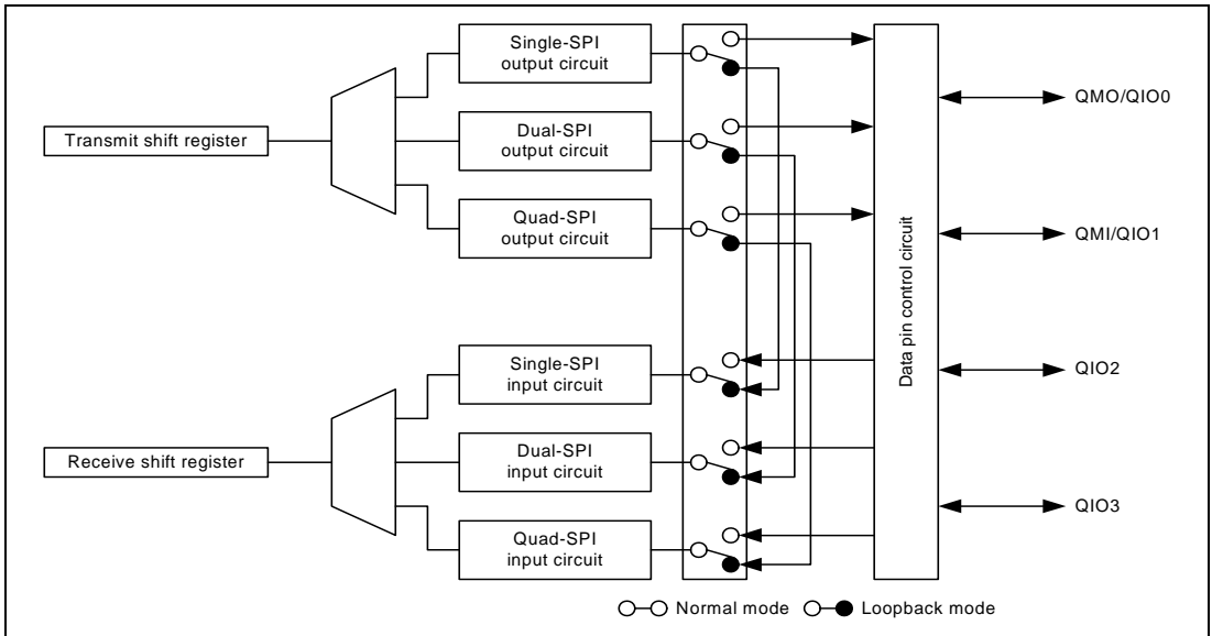
Figure 18.22 Schematic Internal Connection in Loopback Mode
