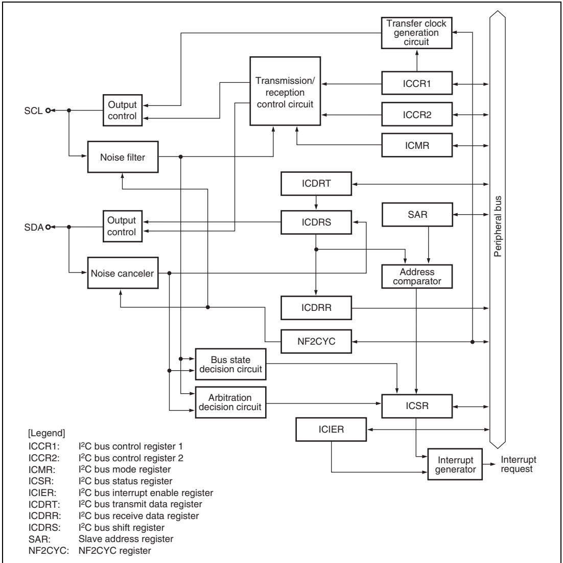
Figure 20.1 Block Diagram
