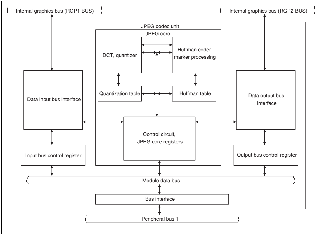
Figure 41.1 Block Diagram
