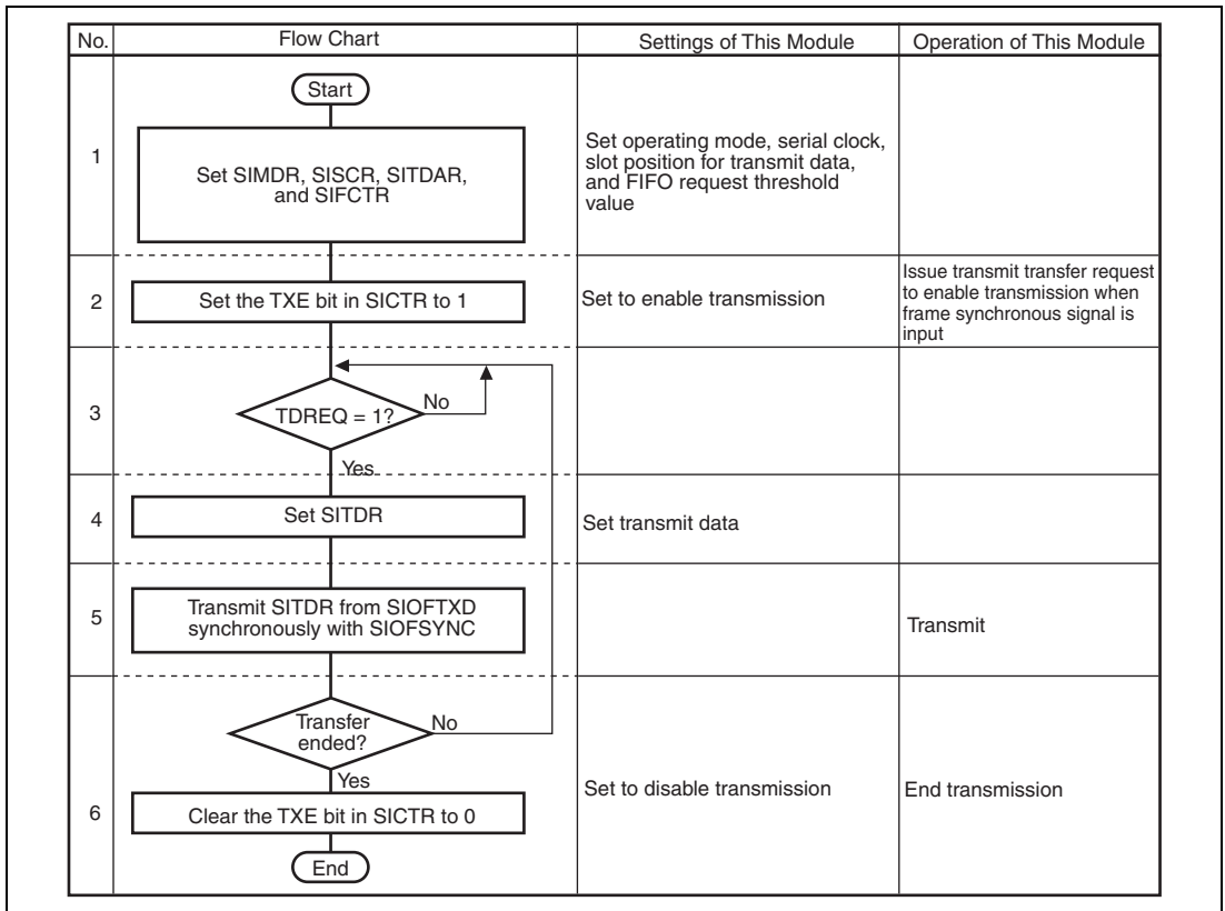
Figure 22.8 Example of Transmit Operation in Slave Mode
