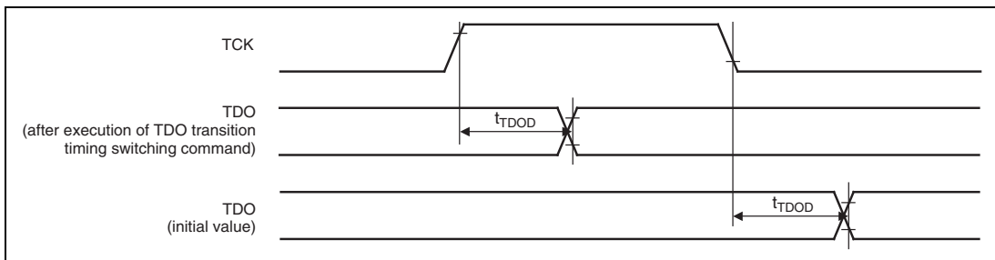
Figure 50.3 User Debugging Interface Data Transfer Timing
