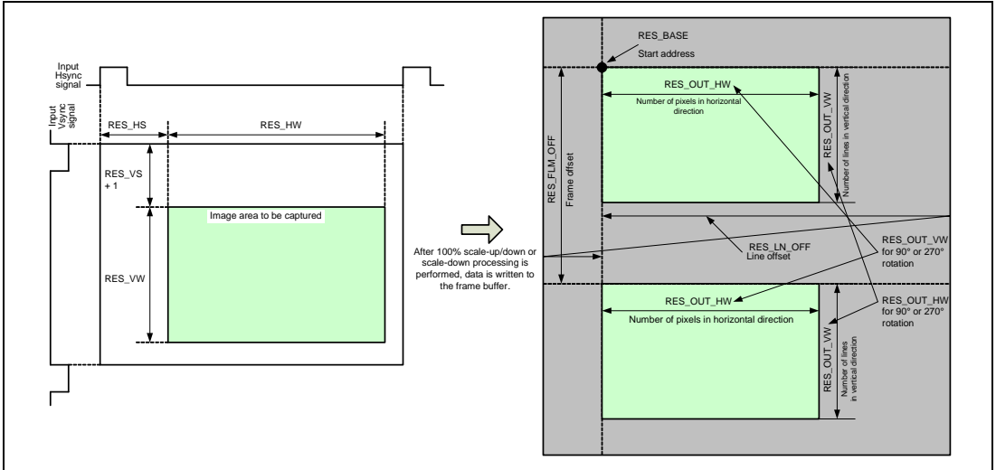
Figure 33.14 Data Arrangement in Frame Buffer
