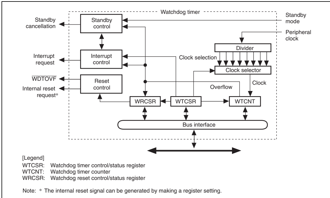
Figure 14.1 Block Diagram
