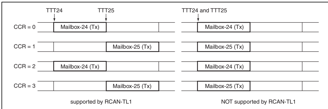
Figure 23.18 Limitation on Tx-Trigger Time
