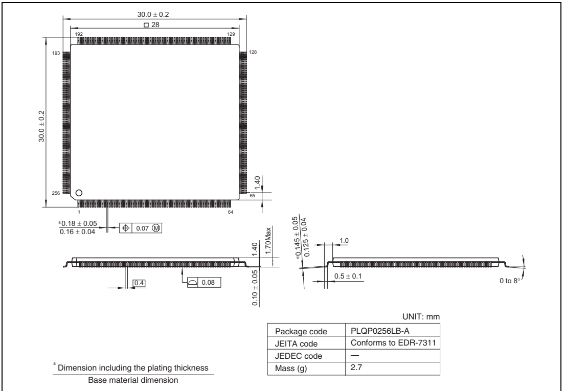
Figure A.2 SH7269 (QFP Version)
