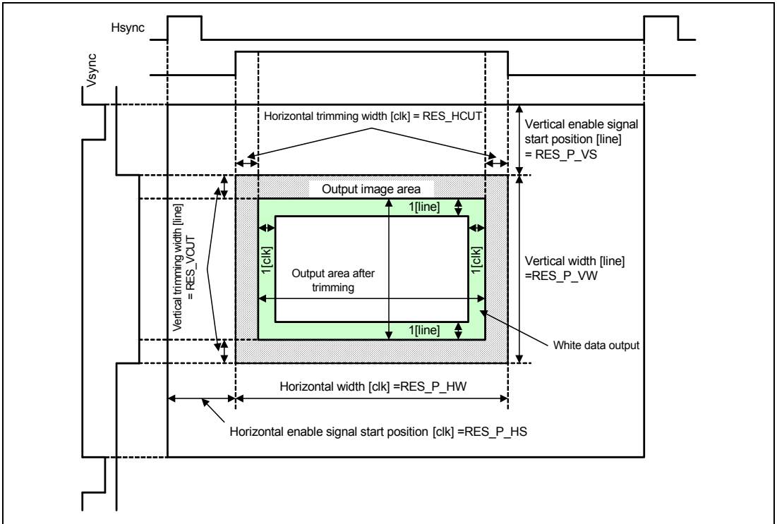
Figure 33.12 Area Relationship for Trimming (Frame Lines Displayed)
