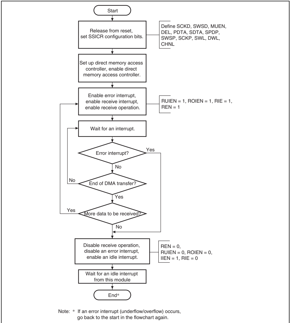
Figure 21.25 Reception Using Direct Memory Access Controller
