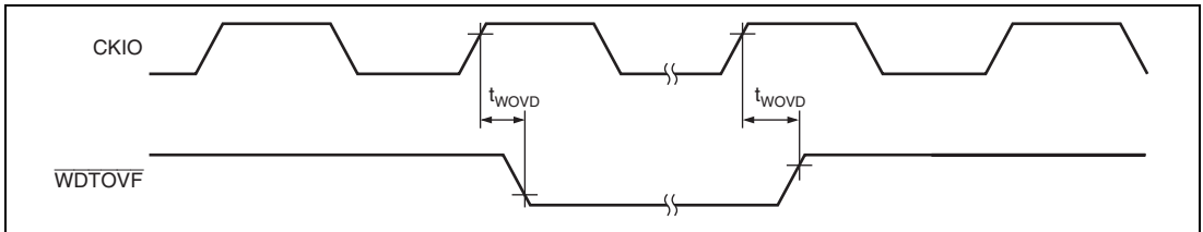
Figure 52.42 \overline{\text{WDTOVF}} Output Timing
