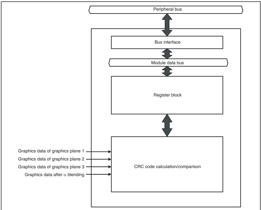
Figure 39.1 Block Diagram
