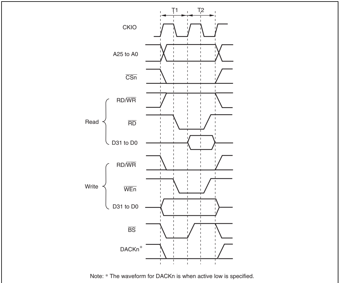
Figure 10.2 Normal Space Basic Access Timing (Access Wait 0)
