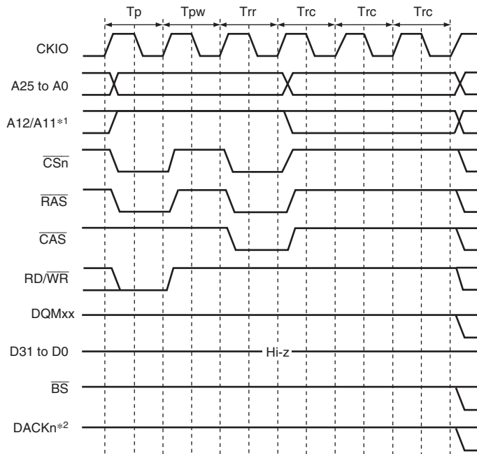
Figure 10.27 Auto-Refresh Timing
