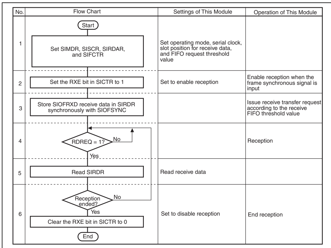
Figure 22.9 Example of Receive Operation in Slave Mode
