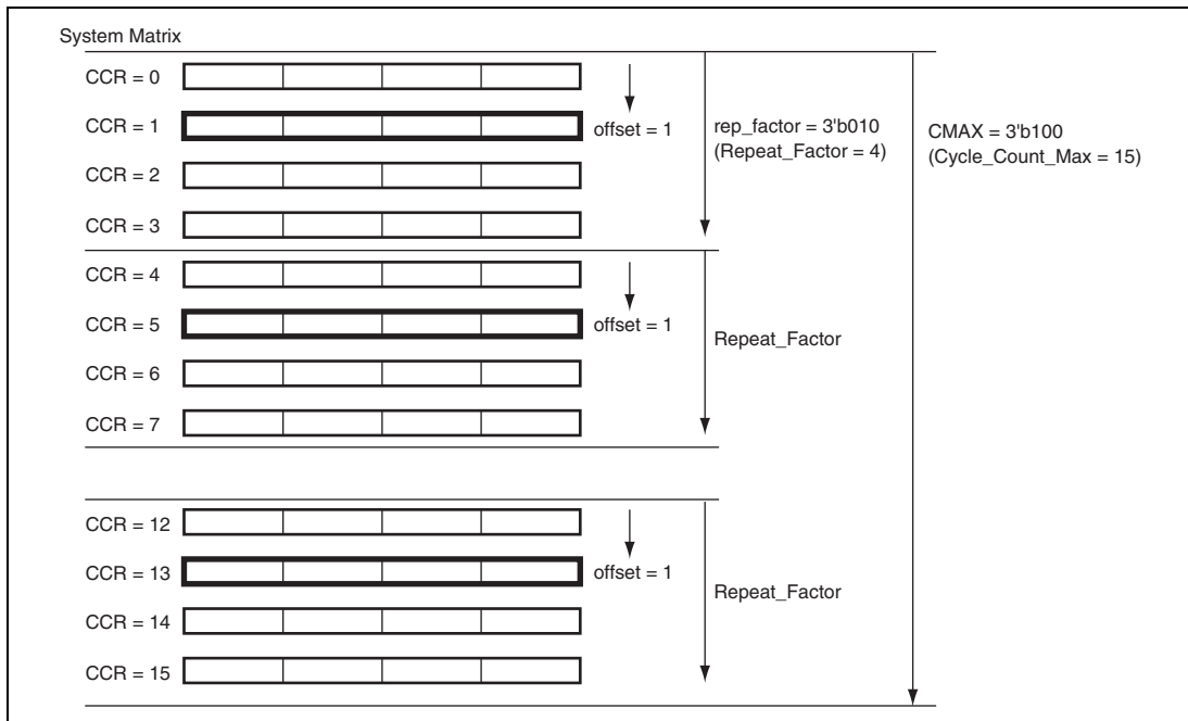
Figure 23.8 System Matrix
