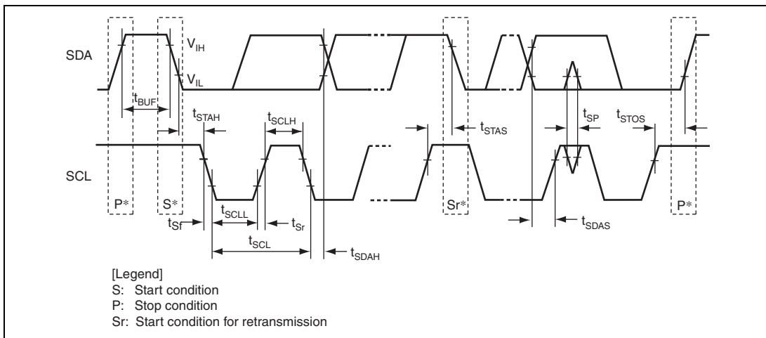
Figure 52.58(1) Input/Output Timing
