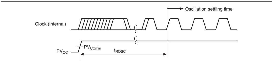
Figure 52.6 Real Time Clock Oscillation Settling Time
