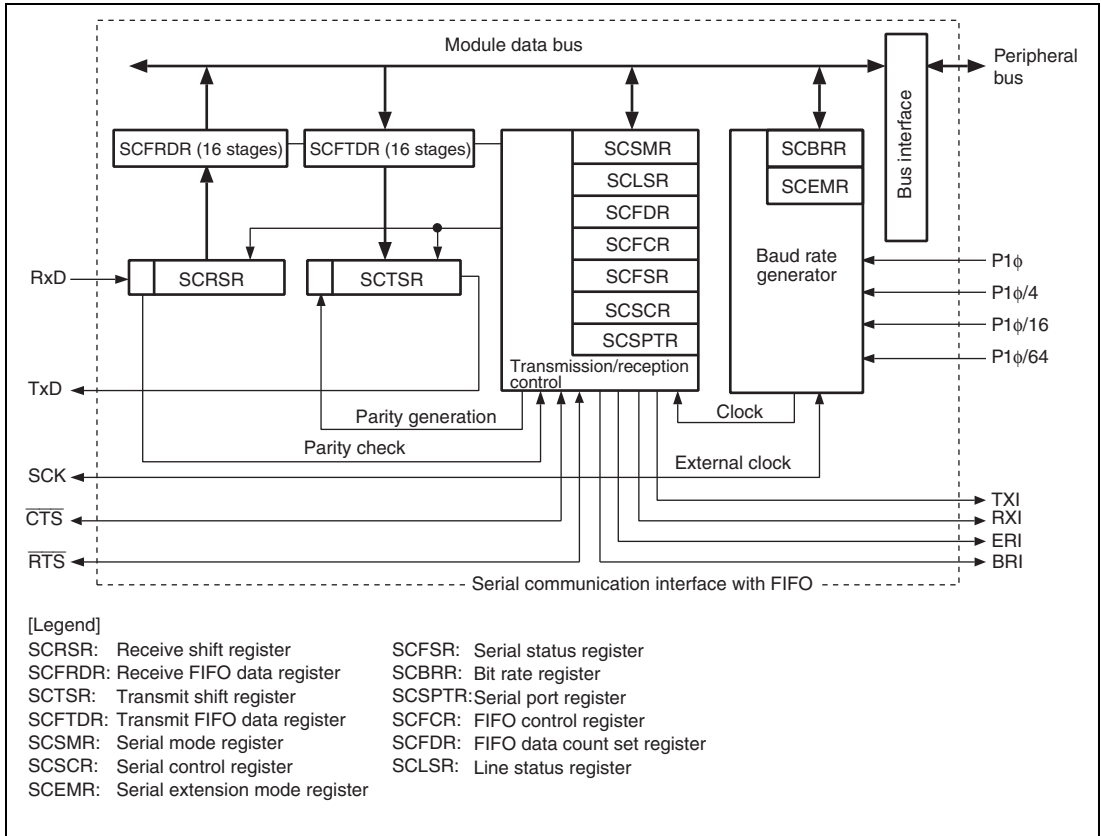
Figure 16.1 Block Diagram
