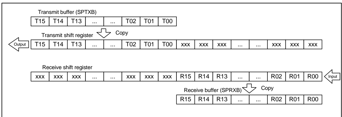
Figure 18.6 MSB First Transfer (16-Bit Data)
