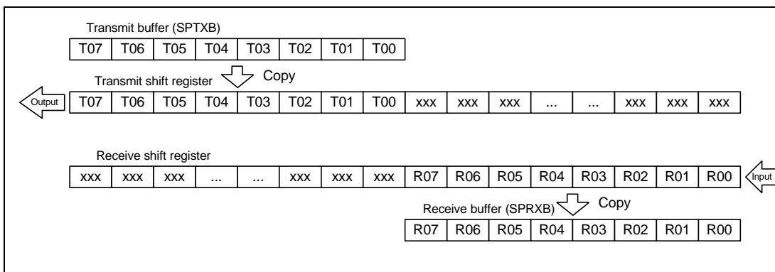
Figure 18.7 MSB First Transfer (8-Bit Data)
