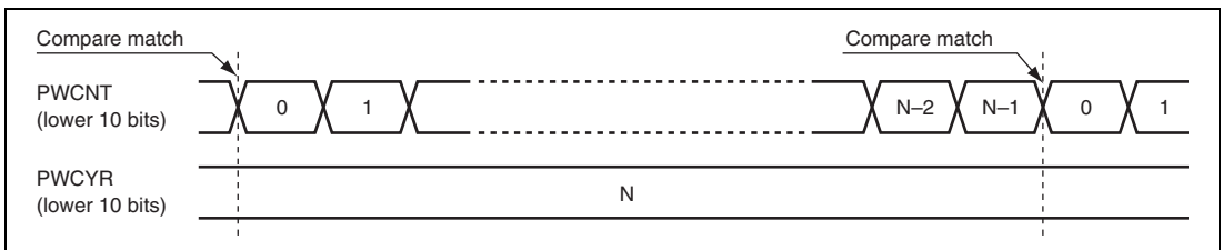
Figure 46.2 Cycle Register Compare Match
