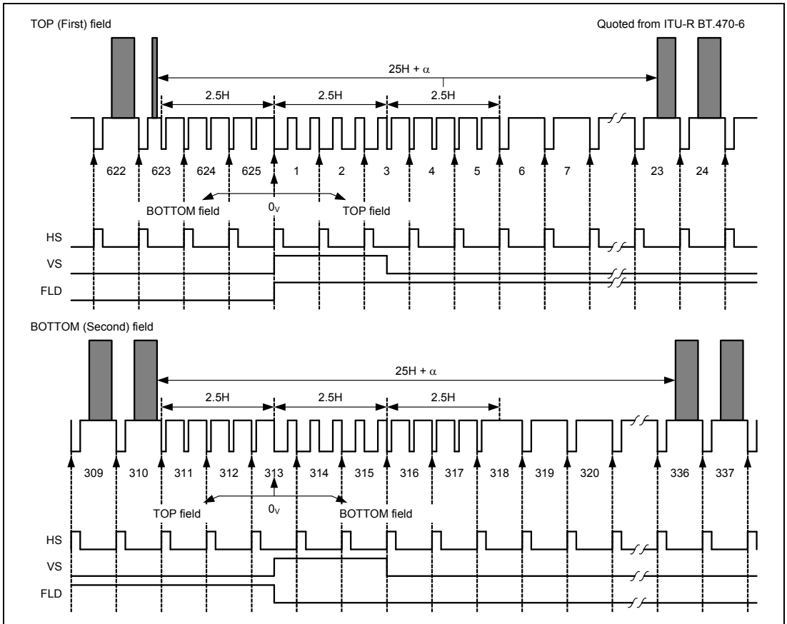
Figure 32.5 BT601 Vertical Timing (625 Lines/50.00 Hz)
