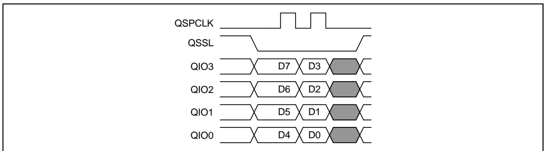
Figure 18.4 Transfer Format in Quad-SPI Format
