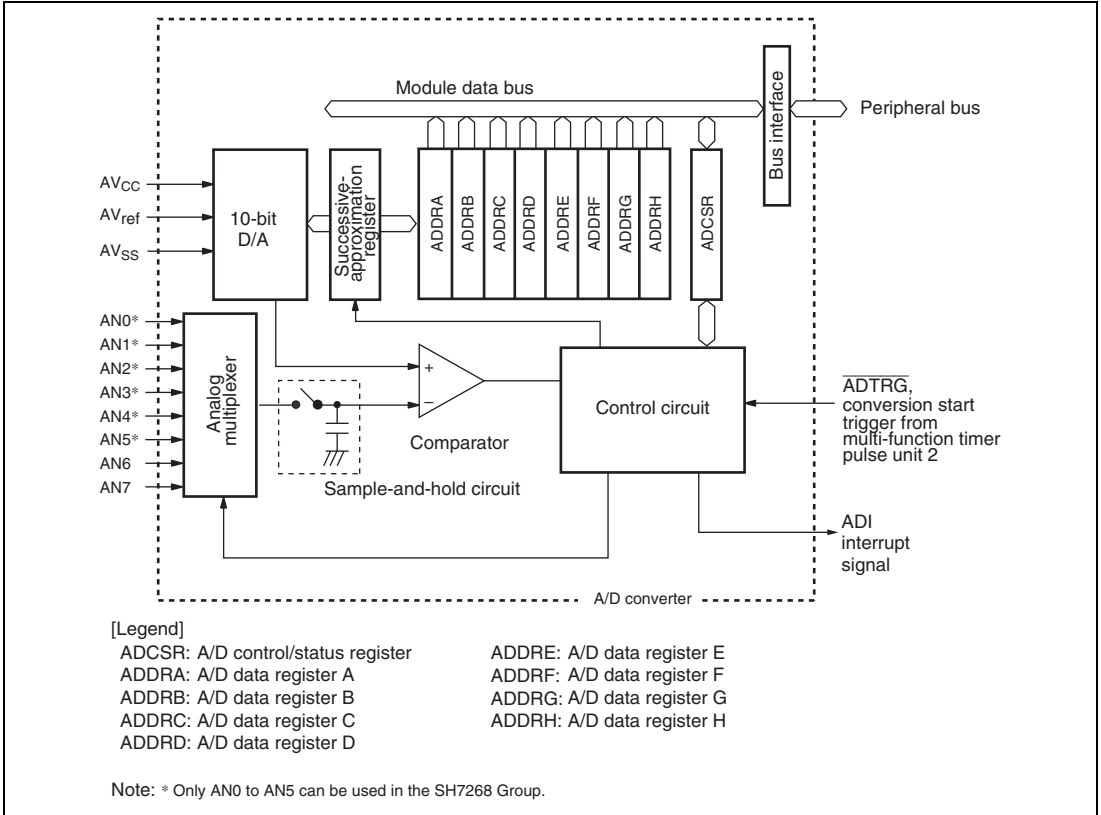
Figure 27.1 Block Diagram of A/D Converter
