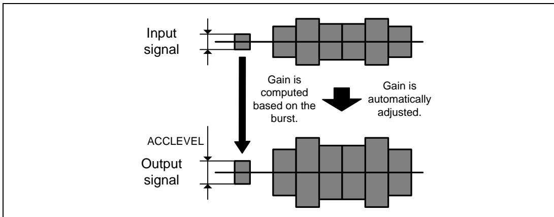
Figure 30.18 ACC Level Setting
