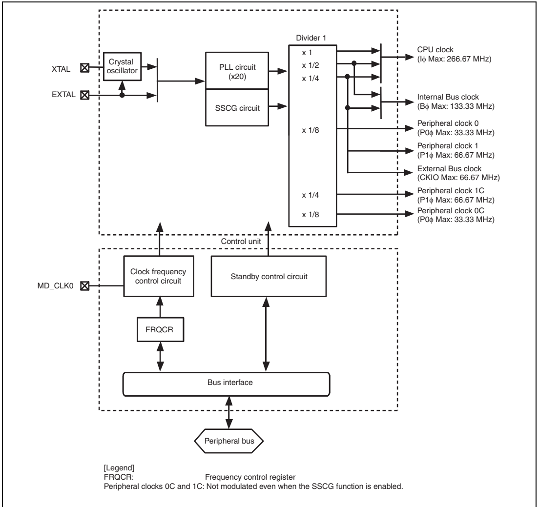
Figure 5.1 Block Diagram
