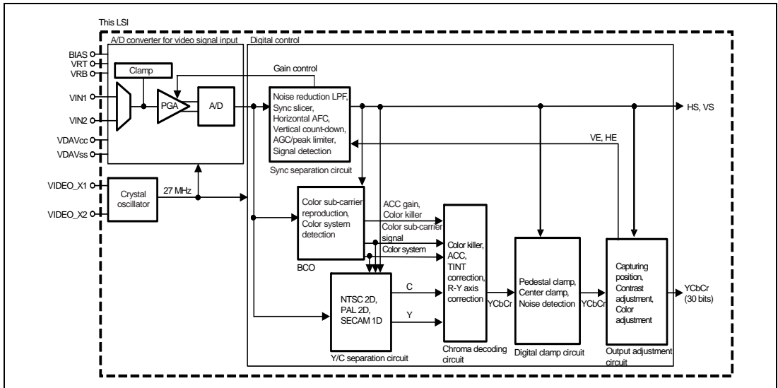
Figure 30.1 Block Diagram
