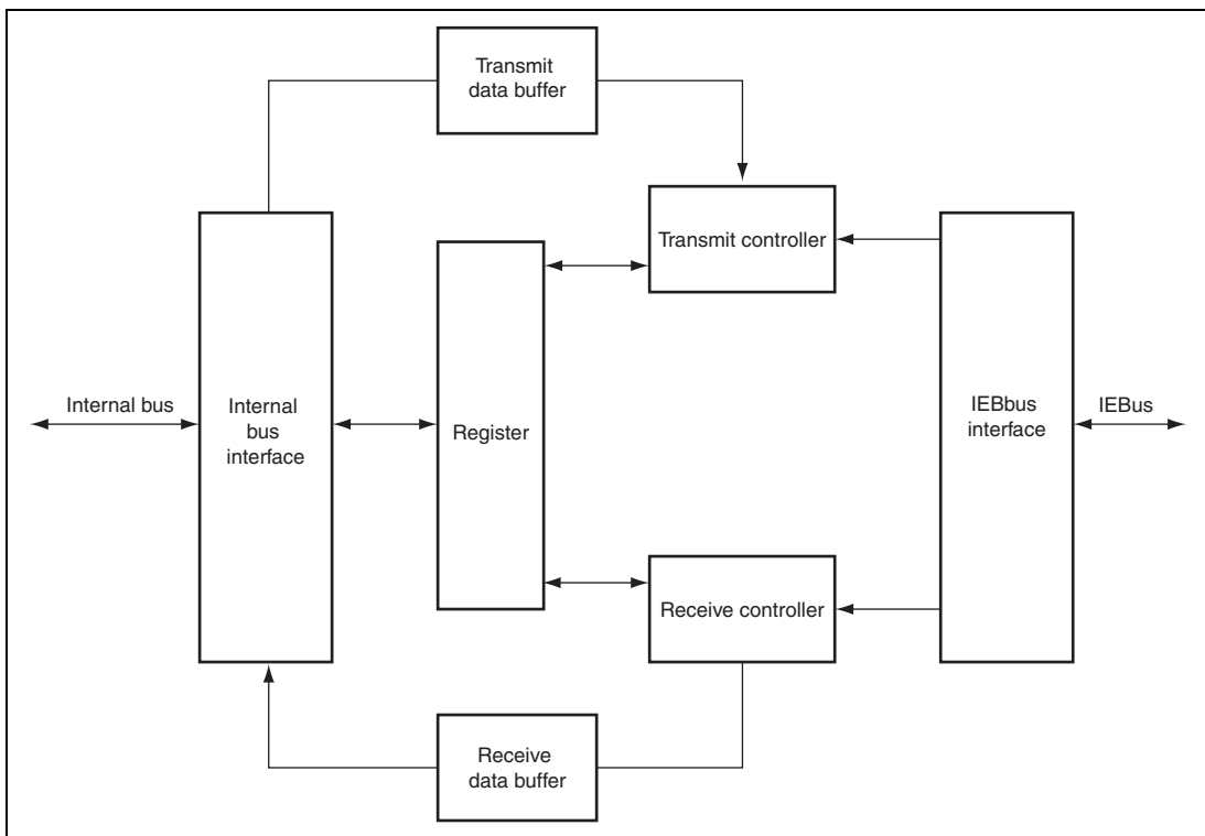
Figure 24.5 Block Diagram
