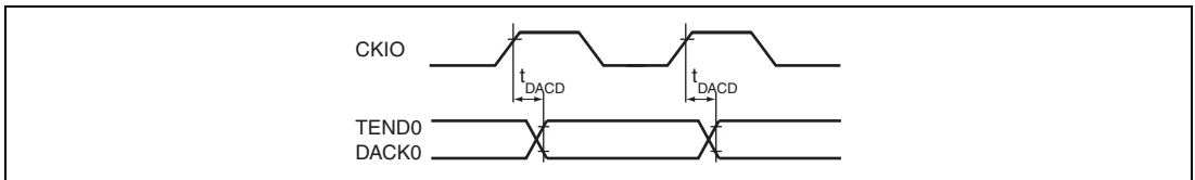
Figure 52.40 DACK, TEND Output Timing
