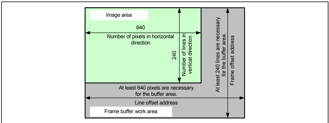
Figure 33.19 Frame Buffer Access Area Setting
