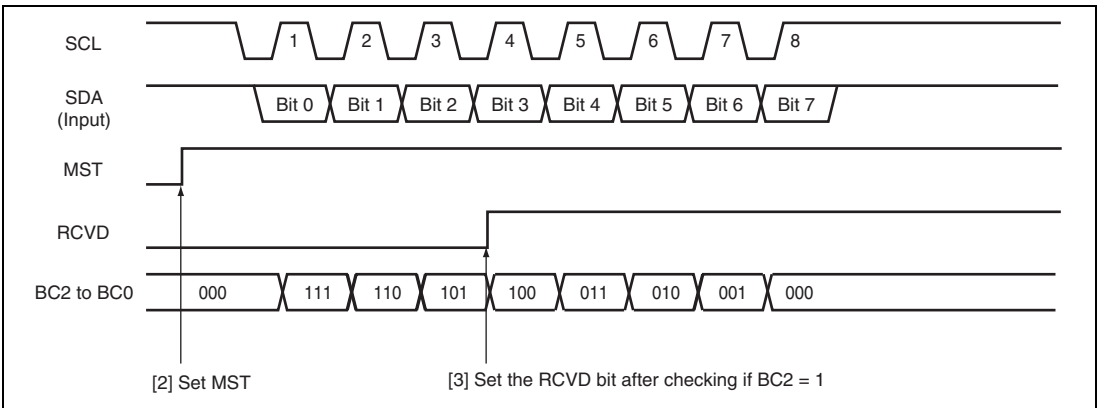
Figure 20.16 Operation Timing for Receiving One Byte (MST = 1)
