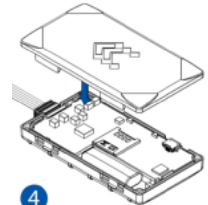
Figure 7 Attaching cover back
