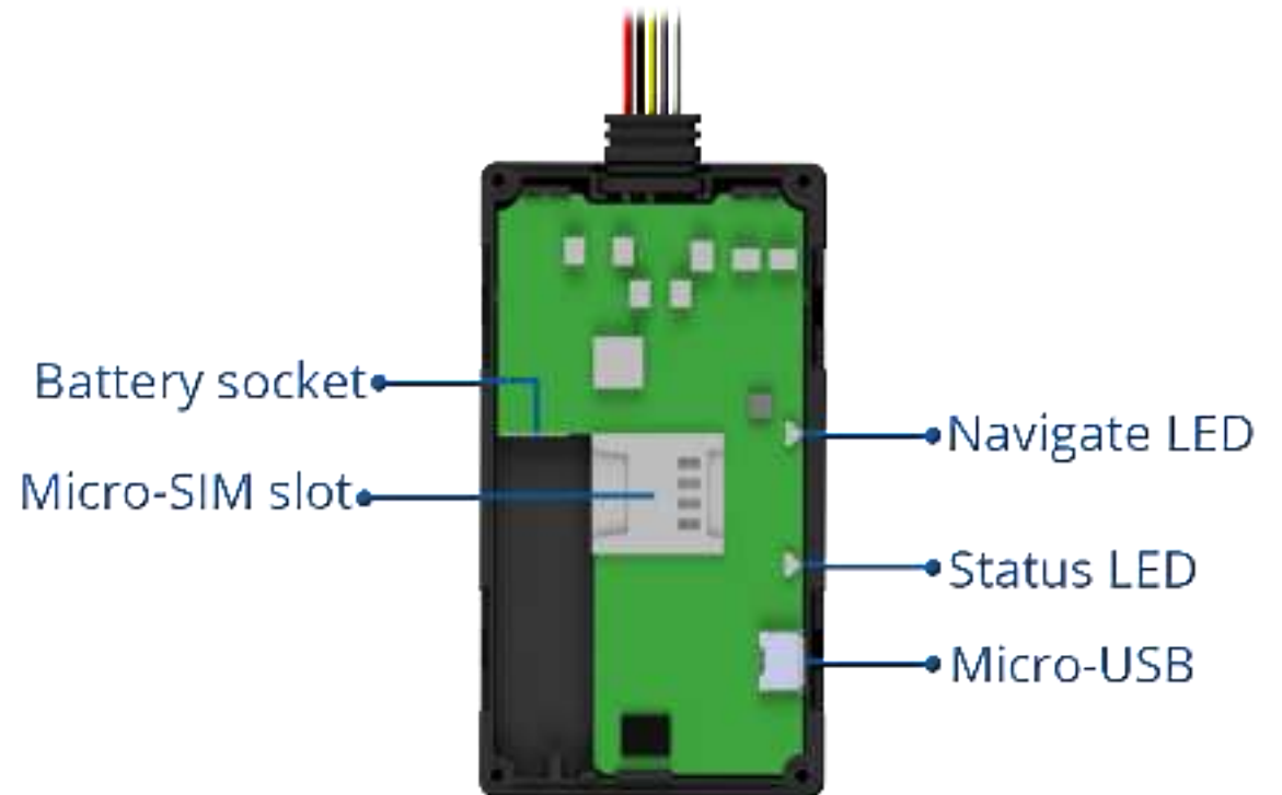
Figure 1 FMB920 device view
