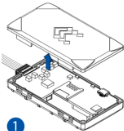
Figure 4 Cover removal
