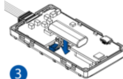
Figure 6 Battery connection
