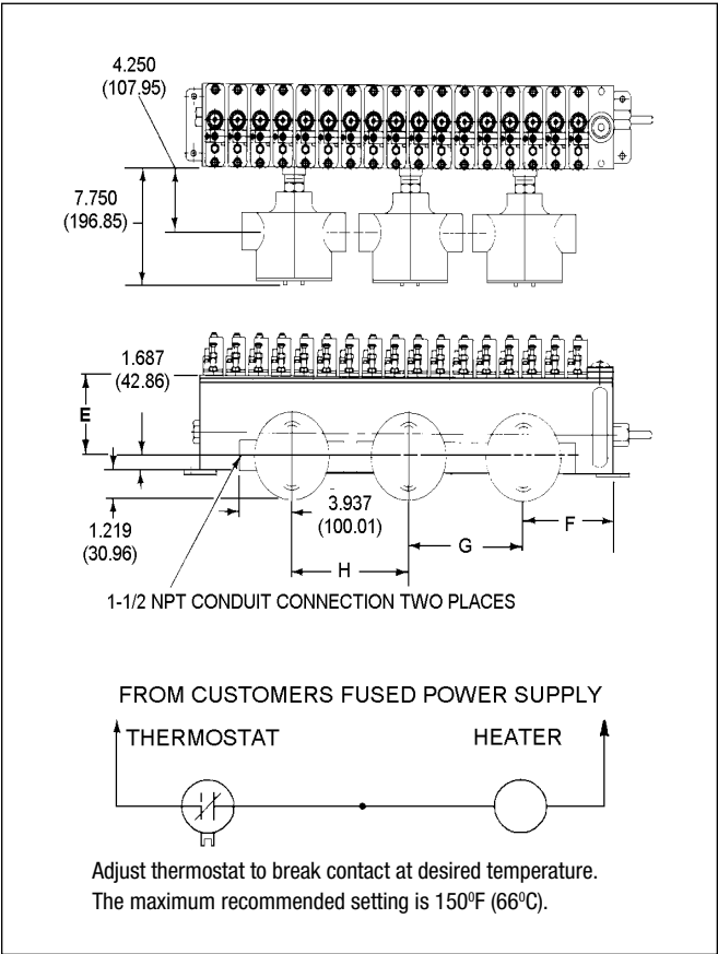
WIRING SCHEMATIC FOR HEATER OPTIONS
