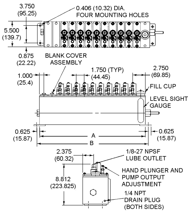
DIMENSIONS SHOWN ARE IN INCHES (MILLIMETERS)
