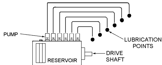
PUMP-TO-POINT SYSTEM
