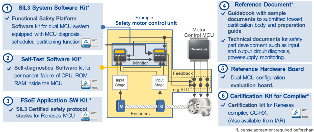
Figure 19: Renesas Functional Safety Solution
