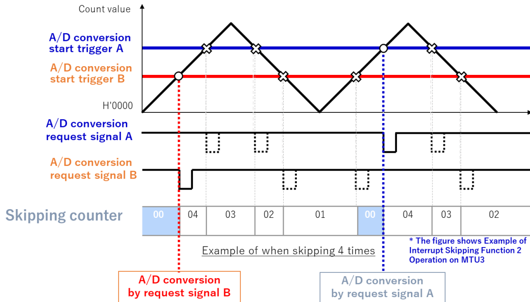
Figure 5: A/D Conversion Thinning Function of Three-Phase Complementary PWM Timer
