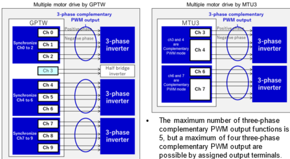
Figure 2: The Number of Three-Phase Complementary PWM Timer
