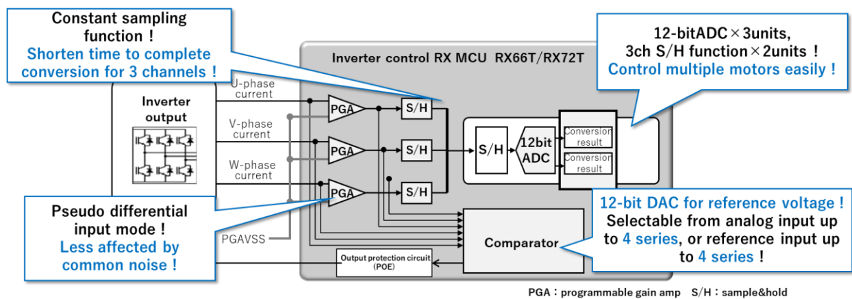
Figure 10: Features of the A/D Converter Equipped in the RX66T/RX72T Series
