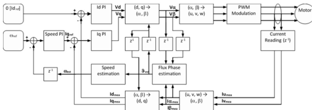
Figure 13: FOC Algorithm Configuration
