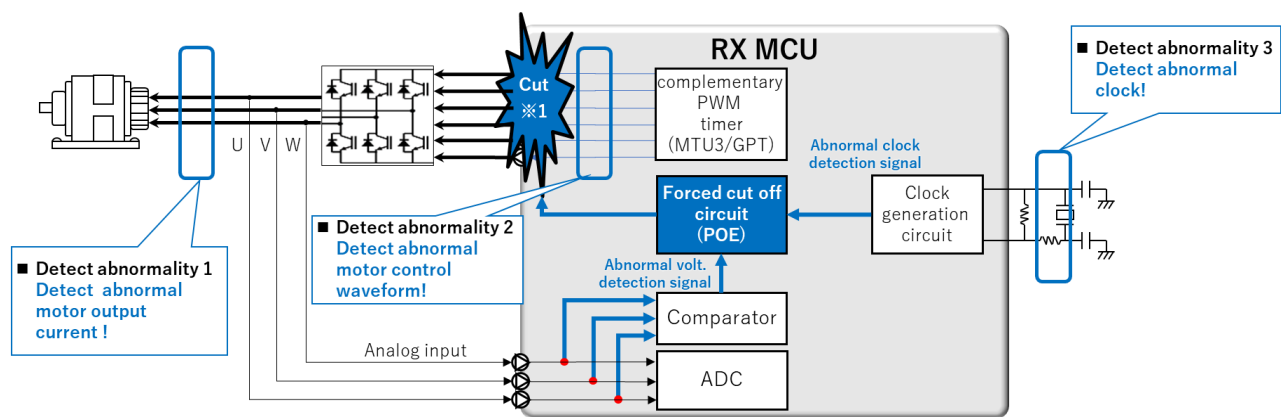
Figure 6: PWM Output Protection Function
