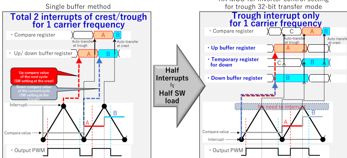
Figure 3: Double Buffer Function of Three-Phase Complementary PWM Timer
