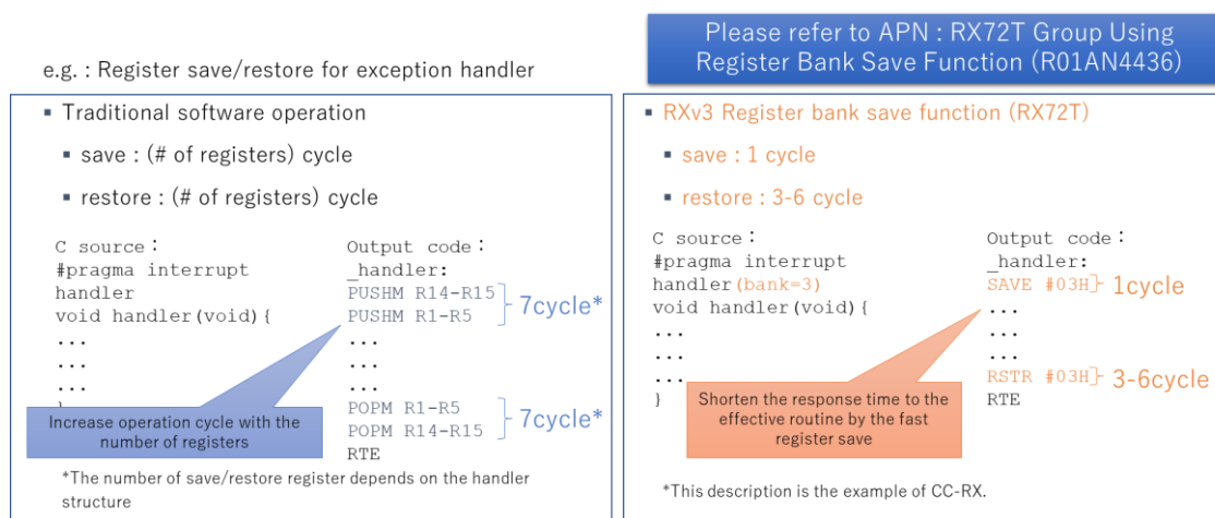
Figure 9: Effect of the Register Bank Save Function – Traditional Microcontroller vs. RX72T
