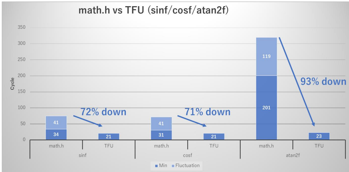
Figure 8: Effect of TFU math.h vs. TFU
