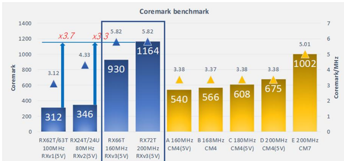
Figure 7: Coremark Benchmark Comparison
