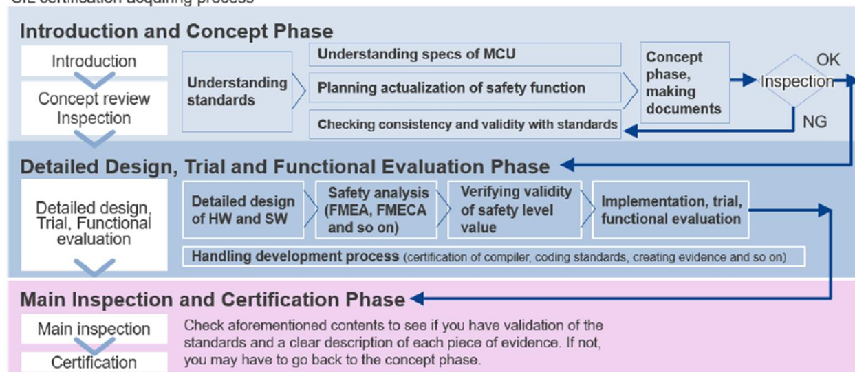
Figure 17: Functional Safety System Development Process
