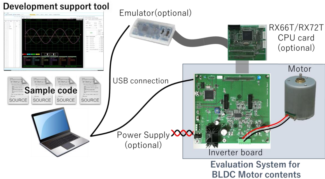
Figure 12: Configuration of Evaluation System for BLDC Motor
