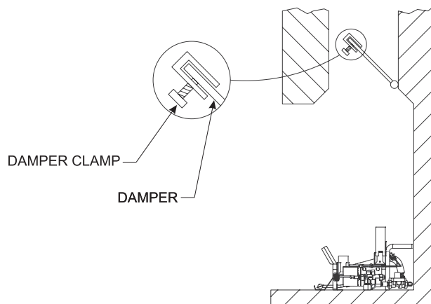
TYPICAL FIREPLACE
