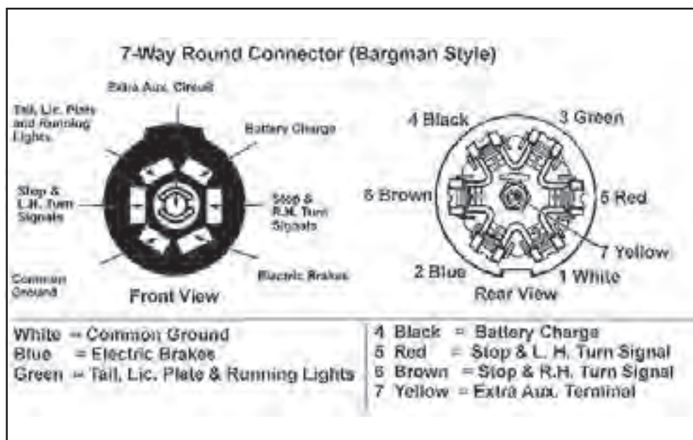
Figure 9-15: Seven-Pin towing connector
