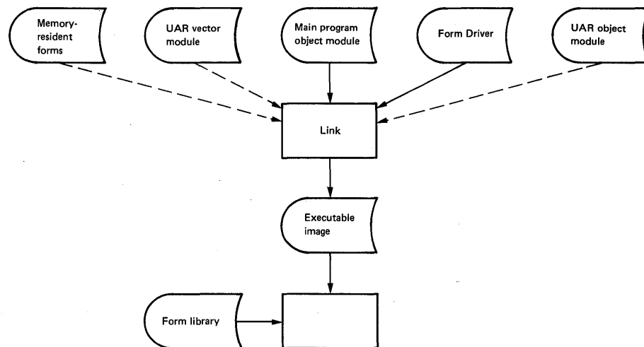
Figure 2-1: Building an Application Program
